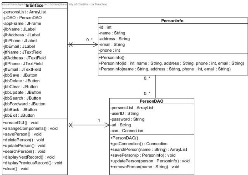
Figure 1.1. An example of a UML class diagram.
