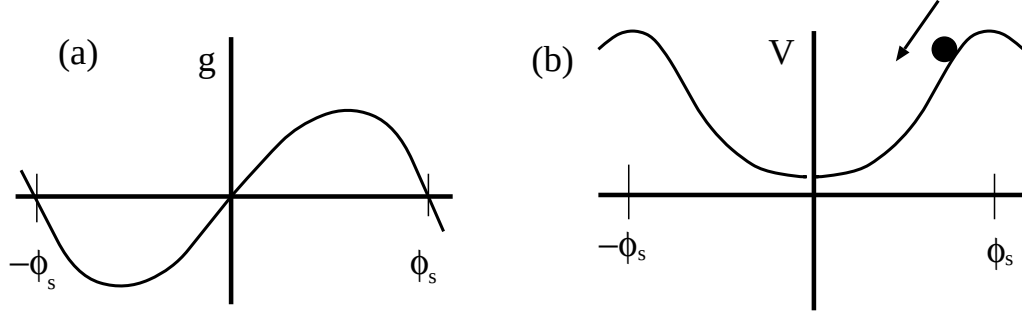
Fig. 9. The functions g and V in the case of front propagation into unstable states. Compare Fig. 4, where the functions are drawn for the case of a front between a stable and a metastable state.
