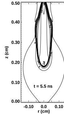
Fig. 1. Examples of three growth patterns: a dendrite in (a), a viscous finger in (b), and streamer in (c). Usually, dendritic growth is studied in liquids with a melting temperature near room temperature. The one shown in (a) was observed in ^3\text{He} [30] at 100 mK, and the fact that it is similar in shape and form to those usually observed illustrates the generality of dendritic growth [courtesy of E. Rolley and S. Balibar]. In (b), a top view of a viscous finger is shown. The air inside the finger like pattern displaces the oil outside (from [31], with permission from the author). The streamer pattern is from a numerical simulation [32].
