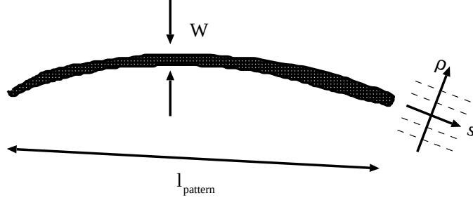
Fig. 8. Qualitative sketch of a curved front of width W , and the local curvilinear coordinate system (\rho, s) used in the derivation of an effective interface model.
