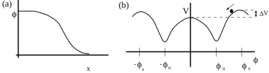
Fig. 5. (a) Example of the type of moving front solution we are looking for. (b) The potential V . A moving front solution like the one sketched in (a) corresponds in the particle-on-the-hill analogy to the solution of the dynamical problem in which the particle starts at the top at \phi_s , moves down the hill and up the one in the center, and comes to rest at the center top as the quasi-time \xi_v \rightarrow \infty .
