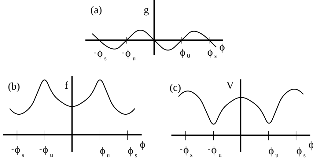
Fig. 4. The function g(\phi) and the associated potentials f(\phi) and V(\phi) used in our discussion of front solutions of Eq. (35)
