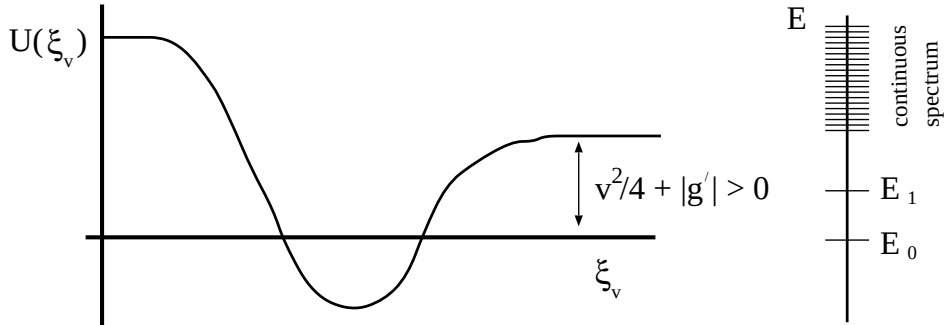
Fig. 7. Sketch of the potential U(\xi_v) which enters in the stability analysis of the front \phi_{v_0} between a stable and a meta-stable state. The asymptotes U(\infty) and U(-\infty) are both positive. The resulting eigenvalues spectrum is sketched on the right. Note that there always is an eigenvalue E = 0 due to the translation mode.
