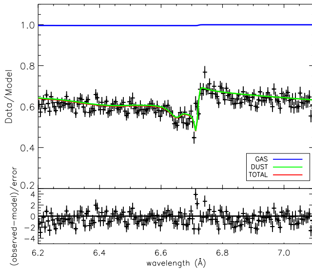
Figure 3.13: Si K-edge GX 17+2.
