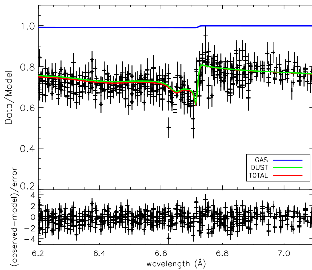
Figure 3.14: Si K-edge 4U 1705-44.
