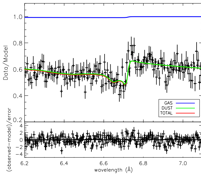
Figure 3.10: Si K-edge 4U 1728-34.
