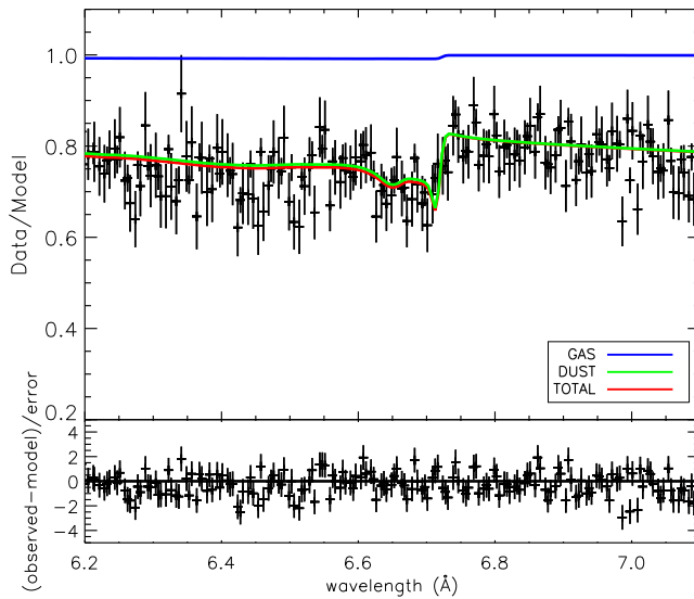
Figure 3.9: Si K-edge 4U 1702-429.
