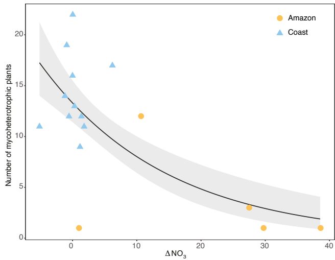
Figure 4 | Relationship between the number of mycoheterotrophic plants observed in the positive plots and the ΔNO 3 (negative plots minus positive plots).
