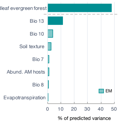
Figure 5 | Ranking of selected predictors explaining the distribution of mycoheterotrophic plants associated with AM and EM fungi as a result of the GLM (above dashed lines) and the hierarchical partitioning analyses (below dashed lines). Predictors are ranked according to the % of predicted variance reflecting their importance in the models. Important predictors are represented as full bars.
