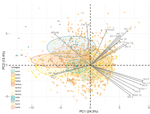
Figure 6 | Principal Components Analysis of the environmental space occupied by mycoheterotrophic plants associated with AM (a) and EM (b) fungi. Only the predictors significantly associated with the first and second principal components are shown. Length of the arrows represent the relative importance of predictors. Clouds of points are the records in the dataset. Ellipses delimitate the environmental space occupied by each lineage.
