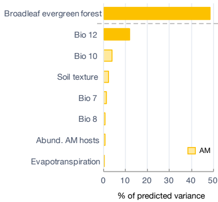
Figure 5 | Ranking of selected predictors explaining the distribution of mycoheterotrophic plants associated with AM and EM fungi as a result of the GLM (above dashed lines) and the hierarchical partitioning analyses (below dashed lines). Predictors are ranked according to the % of predicted variance reflecting their importance in the models. Important predictors are represented as full bars.
