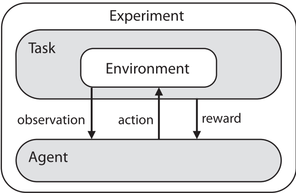
Fig. 11. Overview of the experimental setup for the RL models. The plated components interact with each other according to the arrows to simulate the same trial-and-error learning process that humans undergo.
