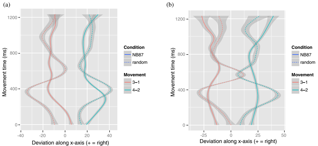
Fig. 6. Averaged trajectories for vertical movements 4-2 and 3-1 between 0 and 1,200 ms after ISI onset. (a) Horizontal deviation during movement (i.e., over time) in early training. Both conditions' trajectories show some centering behavior, bending toward the middle (i.e., right for 3-1, left for 4-2). NB87 trajectories show less deviation. (b) Horizontal deviation during movement in late training. The random condition shows more centering behavior, while the NB87 trajectories show little variation except at the end of the movements when they diverge, showing prediction of the subsequent stimulus.
