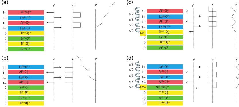
Figure 1.2: (001) LAO / STO heterostructures are made of electrically neutral planes on the STO side and charged planes on the LAO side. (a)–(b) Charge density \rho , electric field E and potential V along the growth direction at the unreconstructed interface with (a) TiO 2 -LaO connection and (b) SrO-AlO 2 connection. (c)–(d) Electronic reconstruction, with (c) half an electron per unit cell transferred to the TiO 2 interfacial plane and (d) half a hole transferred to the interfacial SrO plane, creates electric dipoles at the interface that leads to oscillating electric fields and bounded potentials. Reprinted by permission from Springer Customer Service Centre GmbH: Springer Nature, Nature Materials, N. Nakagawa, H. Y. Hwang and D. A. Muller, Why some interfaces cannot be sharp , Nat. Mater. 5 , 204–9 (2006), Copyright 2015.
