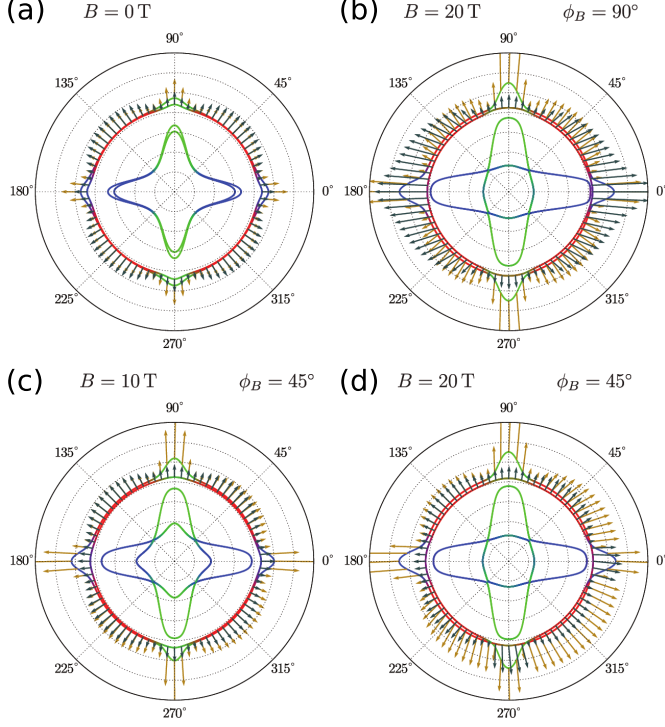
Figure 2.4: Fermi surfaces at n = 2.2 \times 10^{13} \text{ cm}^{-2} for different configurations of the in-plane magnetic field: (a) B = 0 \text{ T} , (b) B = 20 \text{ T} \phi_B = 90^\circ , (c) B = 10 \text{ T} \phi_B = 45^\circ , (d) B = 20 \text{ T} \phi_B = 45^\circ . Magnitude and direction of the vector mean-free-path \Lambda_{\mathbf{k}} as a function of the momentum \mathbf{k} on the outermost bands (which support all of the total conductivity at any fields) are represented by arrows - colors distinguish the two bands of each pair. The longitudinal conductivity \sigma_{xx} is proportional to the average x -component of the vector mean-free-path. (At \phi_B = 0, 90^\circ \rho_{xx} = \sigma_{xx}^{-1} .) The modulation of the vector mean-free-path in (c) is mirror-symmetric with respect to the crystalline axes; therefore \sigma_{xy}(\rho_{xy}) \approx 0 because states with opposite velocities compensate each other with equal weights \Lambda^x . Instead in (d) the texture of the vector mean-free-path is manifestly asymmetric, producing sizable \sigma_{xy} .
