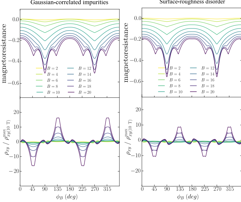
Figure 2.2: (Top) Magnetoresistance \rho_{xx}(B)/\rho_{xx}(0) - 1 and (bottom) transverse resistivity \rho_{xy} (rescaled by the maximum \rho_{xy} at B = 10 \text{ T} ), as a function of the angle between the direction of the magnetic field and the x -axis, at different values of the field-strength. The left panel is for calculations with scattering by Gaussian-correlated impurities, with amplitudes from Eq. (2.4). The right panel is for calculations with scattering by surface-roughness disorder, with amplitudes from Eq. (2.5). The temperature is T = 1 \text{ K} and the density n = 2.2 \times 10^{13} \text{ cm}^{-2} . Other parameters from the first row of Table 2.1 (Sec. 2.8).
