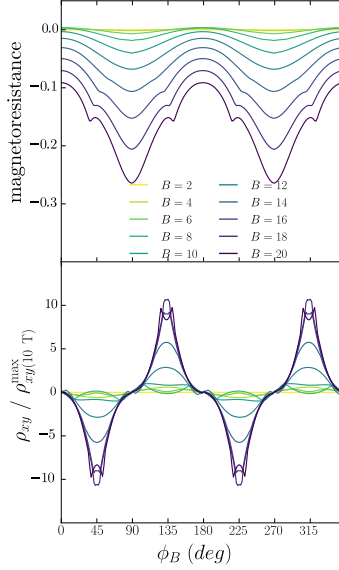
Figure 2.5: Magnetoresistance and transverse resistivity for a negative g -factor (parameters from the second row of Table 2.1).
