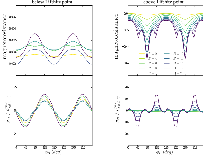
Figure 2.7: Magnetoresistance and transverse resistivity for two different densities (both lower than the density considered in the main text). There is a clear difference in pattern and the magnitude of the anisotropy between the two cases.
