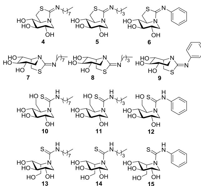
Figure 2. Structures of the new sp^2 -iminosugars prepared in this work.
