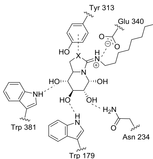
Figure 3. Salt bridge and hydrogen-bonding interactions of compounds 1 ( X = O ) and 2 ( X = S ) in the active site of human GCase as evidenced in the corresponding crystal structures (PDB codes 2XWD and 2XWE) [76]. The proposed sulfur- \pi interaction between the isothioureia S atom of 2 and the aromatic ring of tyrosine 313 is also depicted.
