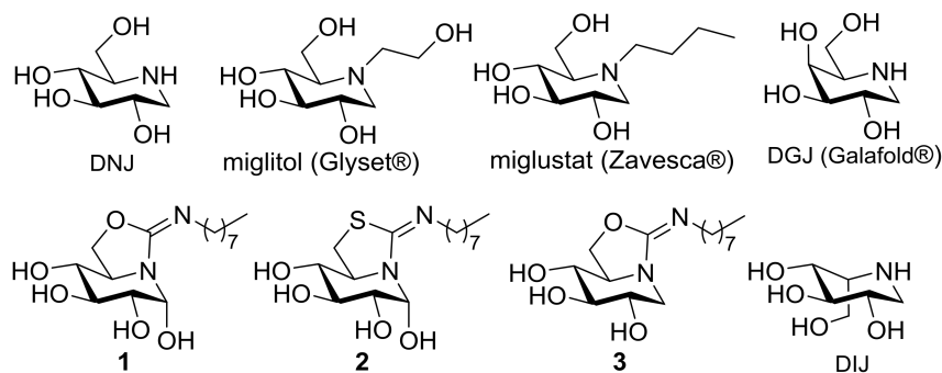
Figure 1. Structures of the iminosugars 1-deoxynojirimycin (DNJ), 1-deoxygalactonojirimycin (DGJ) and 1-deoxy-L-idonojirimycin (DIJ), the DNJ-related drugs miglitol and miglustat, and the sp 2 -iminosugars 1–3.
