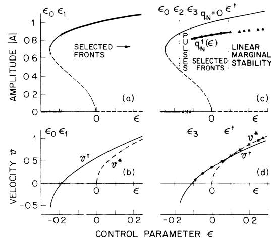
FIG. 1. (a),(c) Bifurcation diagrams and (b),(d) front velocity as a function of control parameter. (a) and (b) refer to the real GL equation [ c_1 = 0 in (1)], which is bistable in the range \epsilon_0 < \epsilon < 0 . Dashed lines refer to unstable solutions, solid lines to stable ones. For \epsilon > \epsilon_1 = -\frac{3}{16} the selected front [thick line in (a)] has velocity v^+ > 0 which is larger than the velocity v^* given by linear marginal stability [dot-dashed line in (b)]. For \epsilon = \epsilon^* = \frac{1}{4} (not shown) v^* = v^+ and for \epsilon > \epsilon^* the linear front is selected. For \epsilon < \epsilon_1 , v^+ < 0 , the |A| = 0 state invades the |A| \neq 0 one [thick line in (a)]. (c) and (d) refer to the complex case [ c_1 = -0.1 , c_3 = 0.2 , c_5 = 0.15 in (1)], for which the front with velocity v^+ and wave vector q_N^+ is selected in the range \epsilon_3 < \epsilon < \epsilon^+ . Solid circles are results of numerical solution of (1). For \epsilon > \epsilon^+ , v^* > v^+ , and we have linear marginal stability (solid triangles), whereas for \epsilon < \epsilon_3 , v^+ < 0 and stable pulses, denoted by crosses, are found for \epsilon_2 < \epsilon < \epsilon_3 . For \epsilon < \epsilon_2 the |A| = 0 state invades all A \neq 0 states.
