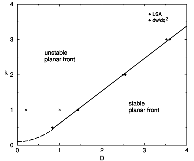
FIG. 3. Stability diagram for parameters D and k . Filled circles show where the region of stability of planar fronts starts as determined by a numerical linear stability analysis, filled diamonds show the same boundary as obtained from the solvability formula for d^2\omega/dq^2|_{q=0} derived in Sec. III C. For k=0.5 both methods give the same value up to the size of the symbol. The solid line is there to guide the eye, the dashed line hints at the fact that while we expect the line of D_c(k) to approach the origin we do not know the precise analytic behavior of D_c(k) for k \rightarrow 0 , since for k=0 the planar front is stable for all D [24,23]. The two crosses represent the simulation performed by Kitsunezaki [22]. For D=0.2 the front in these simulations was unstable, which is consistent with our analysis. For D=1.0 the planar front was stable, which does not agree with our analysis. The probable cause of this apparent discrepancy is discussed in the main text.
