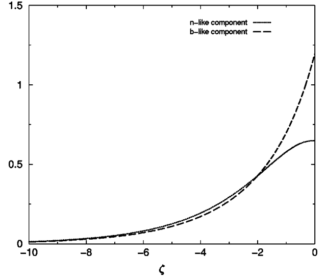
FIG. 12. Zero right eigenvector \bar{\Psi}^{(2)} of the adjoint operator \mathcal{L}^* for k=2 and D=0.3 . The b -like component \Psi_1 approaches a finite value at \zeta=0 with a finite slope; it generally has a higher-order singular term \sim (-\zeta)^{(1+D/k)} .
