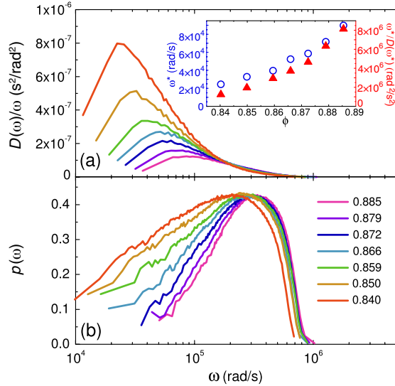
FIG. 4 (color online). (a) D(\omega)/\omega and (b) participation ratio vs \omega as a function of packing fraction [as labeled in (b)]. Inset to (a): the boson peak frequency \omega^* (circles, left) and inverse peak height \omega^*/D(\omega^*) (triangles, right) vs \phi .
