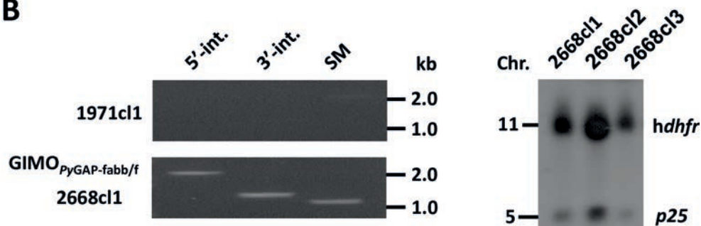
Figure 1. Generation and genotype analysis of the P. yoelii GAP GIMO parent line (GIMO PyGAP-fabb/f ) for introduction of adjuvant-expression cassettes. (A) Schematic representation of the introduction of the hdhfr-yfcu selectable marker (SM) cassette into the fabb/f gene locus of the parent P. yoelii parasite (line 1971cl1). Construct pL2138 contains the hdhfr-yfcu SM flanked by the hsp70 promoter region and the 3' pbdhfr UTR. This construct is integrated into the fabb/f locus by double cross-over homologous recombination at the fabb/f homology regions (HR1, HR2). Positive selection with pyrimethamine selects for parasites that have the fabb/f coding sequence replaced by the SM cassette, thereby creating a GAP GIMO line (2668cl1) for introduction of adjuvant expression cassettes. Location of primers used for PCR analysis and sizes of PCR products are shown. (B) Diagnostic PCR (left panel) and Southern analysis of PFG-separated chromosomes (right panel) confirm correct integration of construct pL2138 in parasites of line 2668cl1. PCR shows the presence of the hdhfr::yfcu marker. 5' integration PCR (5'-int; primers p1/p2), 3' integration PCR (3'-int; primers p5/p6), hdhfr::yfcu (primers p3/p4). Primer locations and product sizes are shown in A and primer sequences in Table S1). Hybridization of PFG-separated chromosomes with a mixture of two probes (the hdhfr probe and a control probe recognizing p25 gene on chromosome 5) shows the presence of the SM cassette marker in the fabb/f -locus on chromosome 11 in three clones of the 2668 line.
