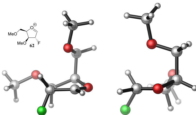
Figure 6. Ball-stick model of the ^4E conformation of 2-fluoroxylidose oxocarbenium ion 62 , viewed through the C-2–C-3 bond and C-1–C-2 bond respectively.
