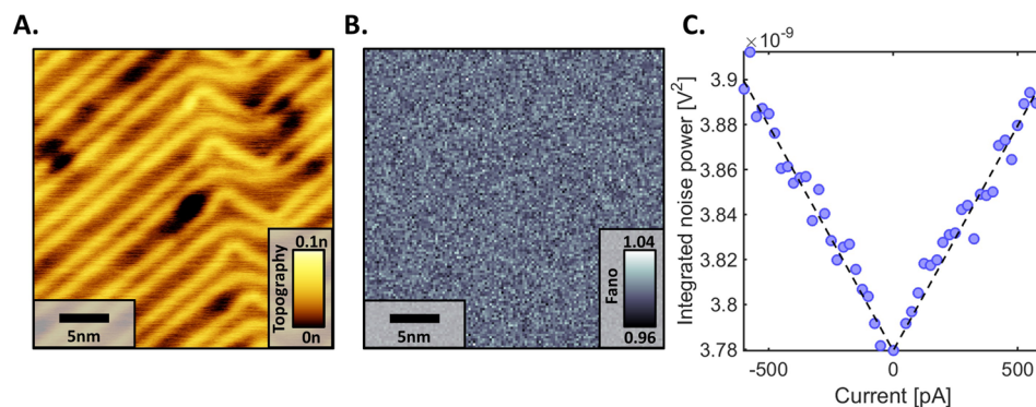
FIG. 4. Benchmark of noise-sensitive measurements on gold on a mica sample. (a) An atomically resolved STM topographic image of the Au(111) surface on a 30 nm field of view; the “herringbone” reconstruction is clearly visible. (Setup condition bias: 100 mV, current set point: 100 pA). (b) Spatially resolved noise map at 500 mV, 500 pA in the same field of view as (a), acquired in 48 h. It shows homogeneous Poissonian (Fano = 1) noise at all locations. Here the Fano factor is extracted as F_{\text{measured}} = [S(500 \text{ pA}) - S(0 \text{ pA})]/[2e500 \text{ pA}] . (c) Single point noise spectrum acquired at a random location in (b). The tunnel junction resistance is kept fixed to 1 \text{ G}\Omega .
