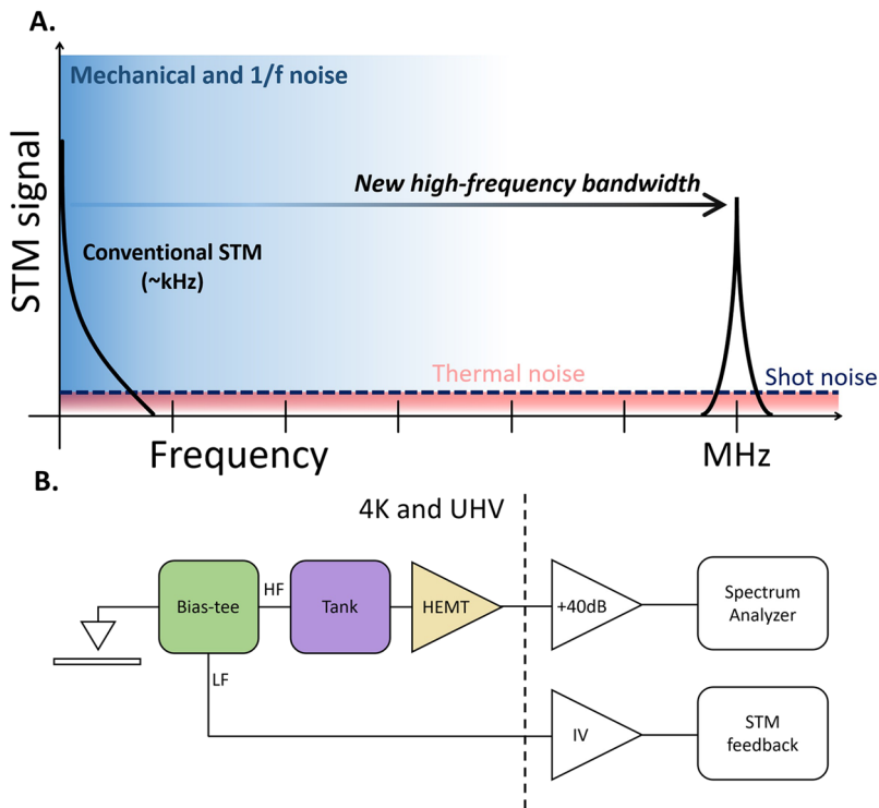
FIG. 1. Noise in scanning tunneling microscopy (STM). (a) The different noise sources in STM and their frequency dependence are depicted in this schematic plot. At low frequencies, mechanical and 1/f noise dominate (indicated by the blue region), and in this region, conventional STM is sensitive. To measure shot noise in the tunnel junction, we need to create a new bandwidth at high-frequency. Here thermal noise and shot noise are the most dominant noise sources since they are independent of frequency. (b) Requirements for the newly built amplifier for combining STM and noise-spectroscopy. Crucial components are highlighted: (i) the bias-tee (green) that separates the low and high frequency signals. (ii) Tank circuit (purple). (iii) High electron mobility transistor (HEMT, indicated in yellow) to amplify the high-frequency signal. Both the low and high frequency signals have additional room temperature amplification and detection (white).
