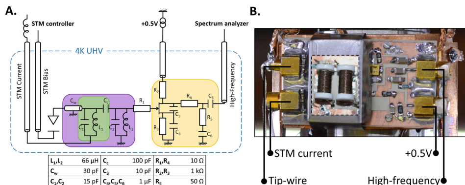
FIG. 2. Newly developed amplifier for scanning noise spectroscopy. (a) Circuit diagram of the amplifier. The colored boxes (green, purple, and yellow) highlight specific parts of the amplifier corresponding to Fig. 1(b). (b) Photograph of the printed circuit board. The niobium inductors are covered by a niobium shield.
