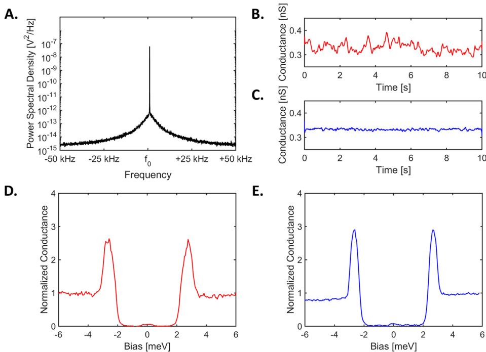
FIG. 5. MHz differential conductance. (a) Power spectrum obtained around the resonance peak. The modulation signal for the lock-in measurement is applied at the resonance frequency (3.009 MHz). (b) Differential conductance measured over time at 887 Hz. A voltage modulation of 0.5 mV is used, and feedback is disabled. (c) Differential conductance measured over time at the resonance frequency (3.009 MHz) under similar conditions as (b). (d) Differential conductance spectrum obtained with a 0.5 mV voltage modulation at 887 Hz (time constant 2 ms) on a Pb(111) surface at a base temperature of 3.3 K. (e) Differential conductance spectrum obtained at the resonance frequency (3.009 MHz, time constant 3.5 \mu s) obtained under the same conditions as (d).
