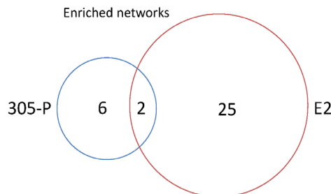
Supplementary Figure S5 – Venn diagram of Ingenuity Pathway analysis of ER \alpha S305-P only, E2 only and overlapping gene sets (See Suppl. Table 5)
