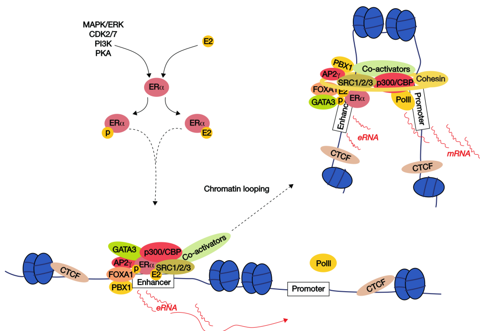
Figure 1: The Estrogen Receptor \alpha transcriptional complex pathway. When activated by its natural ligand estradiol or by direct phosphorylations, ER\alpha binds to enhancers made accessible by pioneer factors (e.g. FOXA1). A transcriptional complex including p300, CBP, SRCs and other co-activators is assembled and enhancer RNAs are transcribed. After cohesin-stabilized chromatin looping to associated gene promoters, RNA polymerase II (Pol II) is recruited and an active transcriptional complex is formed, capable of transcribing associated genes.
