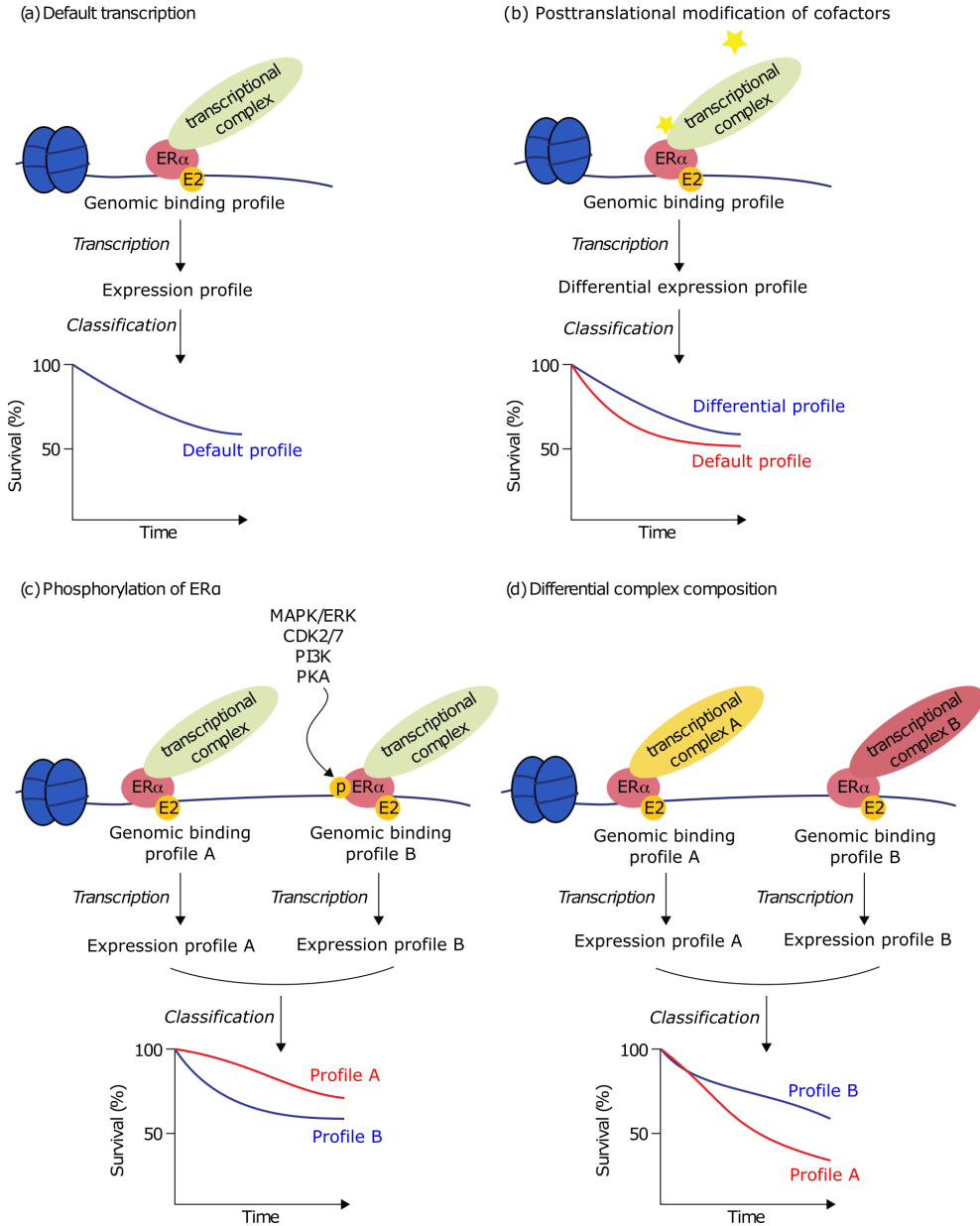
Figure 2: ERα transcriptional complex composition, genomic profile and transcriptional output.
