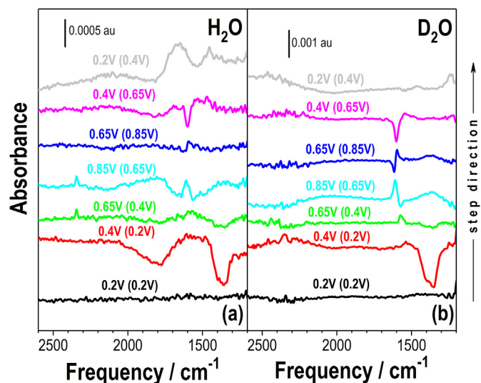
Fig. 3. Infrared spectra recorded for Pt(100) in (a) \text{H}_2\text{O} and (b) \text{D}_2\text{O} , in 0.1 M \text{HClO}_4 + 0.01 M \text{NaNO}_3 . The sample potential is indicated in the legends and the reference potential in brackets. The arrow at the right side of the figure indicates the direction of the steps.
