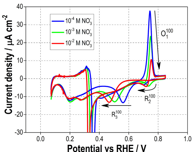
Fig. 4. Cyclic voltammetry ( 5\text{ mV s}^{-1} ) on Pt(100) in 0.1\text{ M HClO}_4 with different concentrations of nitrate. The arrows are used as a guide to the eye for the dependence of the \text{O}_1 , \text{R}_2 and \text{R}_3 peaks as the concentration of nitrate increases.
