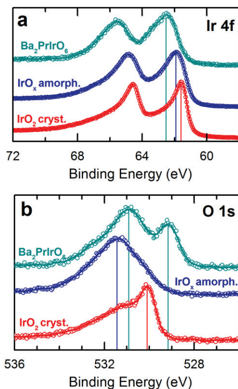
Figure 2. XPS results of pristine \text{Ba}_2\text{PrIrO}_6 , amorphous \text{IrO}_x and crystalline \text{IrO}_2 . (a) Ir 4f and (b) O 1s spectra. Additional results of the leached \text{Ba}_2\text{PrIrO}_6 are presented in the supporting information (Fig. S2).
