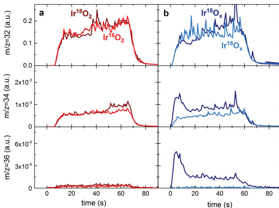
Figure 5. Online observation of lattice oxygen evolution on (a) rutile \text{Ir}^{18}\text{O}_2 / \text{Ir}^{16}\text{O}_2 and (b) hydrous \text{Ir}^{18}\text{O}_x / \text{Ir}^{16}\text{O}_x films during 60 s of anodic polarization at 25 \text{ mA cm}^{-2}_{\text{geo}} . The signals from m/z of 32, 34 and 36 correspond to ^{32}\text{O}_2 , ^{34}\text{O}_2 and ^{36}\text{O}_2 , respectively. Electrolyte: 0.1 M \text{HClO}_4 in \text{H}_2^{16}\text{O} .
