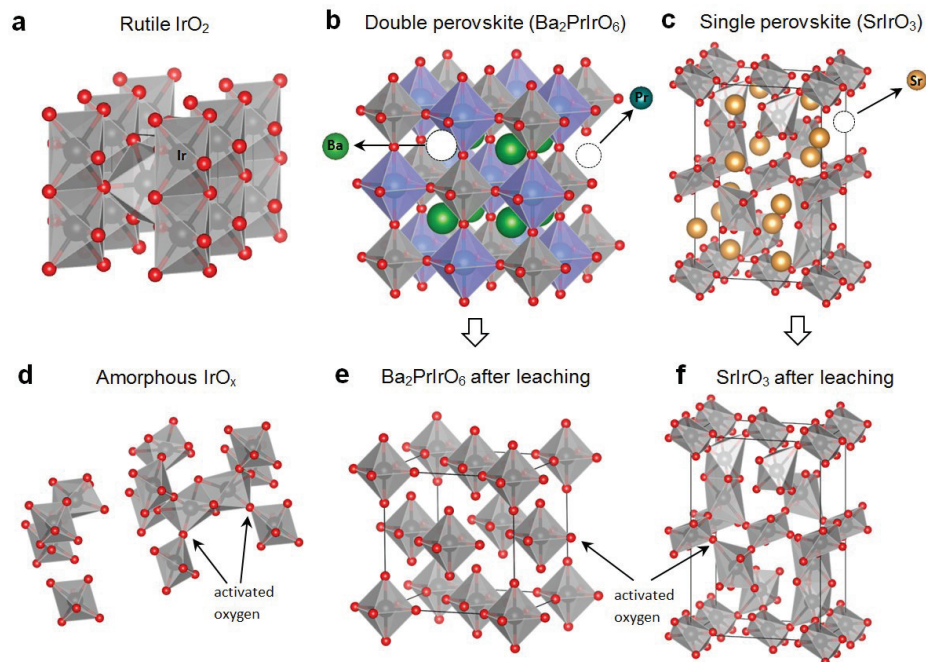
Figure 1. Crystal structure of the investigated materials. (a) rutile IrO 2 ; (b) double perovskite (e.g. Ba 2 PrIrO 6 ); (c) single perovskite (SrIrO 3 ); (d) assumed structure of amorphous iridium oxide, gaps are filled with intercalated water molecules (not shown); (e) leached double perovskite showing isolated IrO 6 octahedra, which will collapse into an amorphous structure; (f) leached SrIrO 3 resulting in an “anatase” iridium oxide structure.
