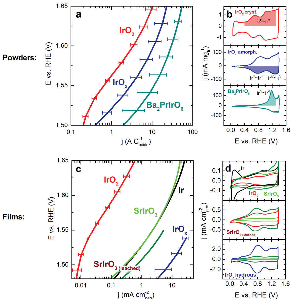
Figure 4. Comparison of the investigated materials in terms of activity. (a) OER-activity of the powder materials recorded with a linear scan of potential at 5 \text{ mV s}^{-1} (iR-drop corrected). The current is normalized to the pseudocapacitive charge in the anodic scan between 0.4 and 1.3 \text{ V}_{\text{RHE}} at 200 \text{ mV s}^{-1} . (b) Cyclic voltammograms recorded with 200 \text{ mV s}^{-1} , the integrated area of the oxide charge used for normalization is highlighted. (c) OER-activity of the investigated films recorded with a linear scan of potential at 5 \text{ mV s}^{-1} . The current is normalized to the geometric surface area. (d) Cyclic voltammograms recorded with 200 \text{ mV s}^{-1} . All measurements were carried out in 0.1 \text{ M HClO}_4 purged with argon.
