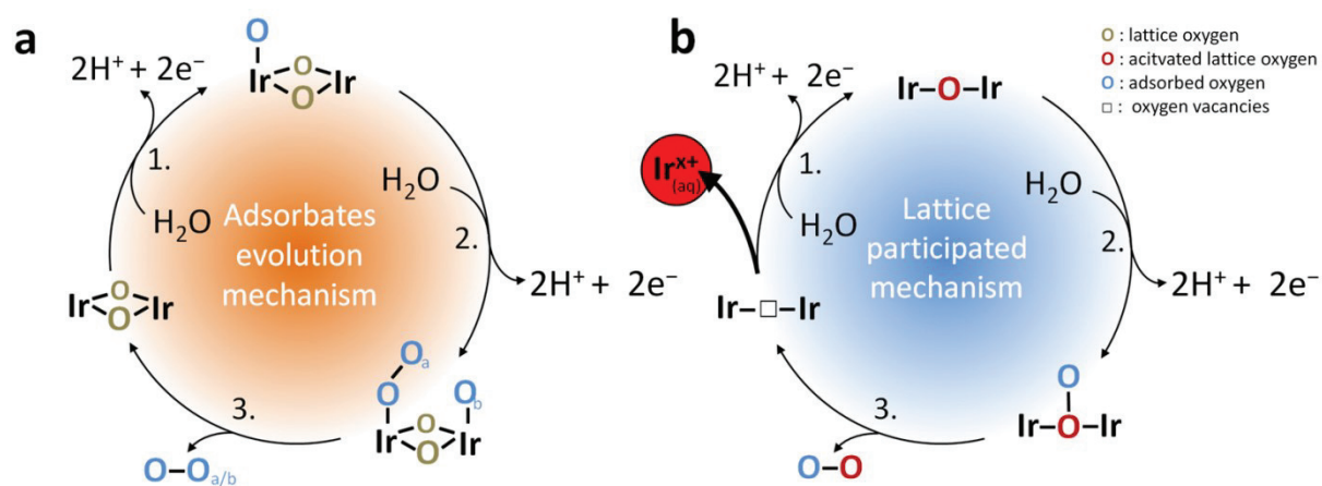
Figure 6. Sketch of the simplified OER reaction mechanism with dissolution pathway. (a) Classical mechanism for crystalline IrO 2 without participation of lattice oxygen. Two possible pathways are presented: single site and double site. (b) Mechanism suggested for amorphous iridium oxide and leached perovskites with participation of activated oxygen in the reaction forming oxygen vacancies. Weakening the binding of iridium in the structure is taken as main reason for enhanced dissolution. To complete the cycle, vacancies can be filled again by adsorption of water. Octahedral configuration of iridium is not presented completely as well as nucleophilic attack of water and removal of proton is merged to one step to not overcrowd the scheme.
