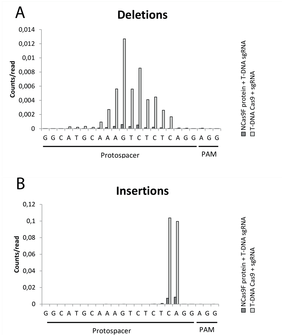
Figure 2. Deletion frequency (A) and insertion frequency (B) for each nucleotide of the PDS target. Deep sequencing analysis of the target sequence obtained from tissue infiltrated with an Agrobacterium transferring NCas9F protein combined with a T-DNA expressing the sgRNA and tissue infiltrated with Agrobacterium transferring a T-DNA expressing both Cas9 and sgRNA. Relative numbers of mutated reads are depicted as a fraction of the total number of reads numbers per position.
