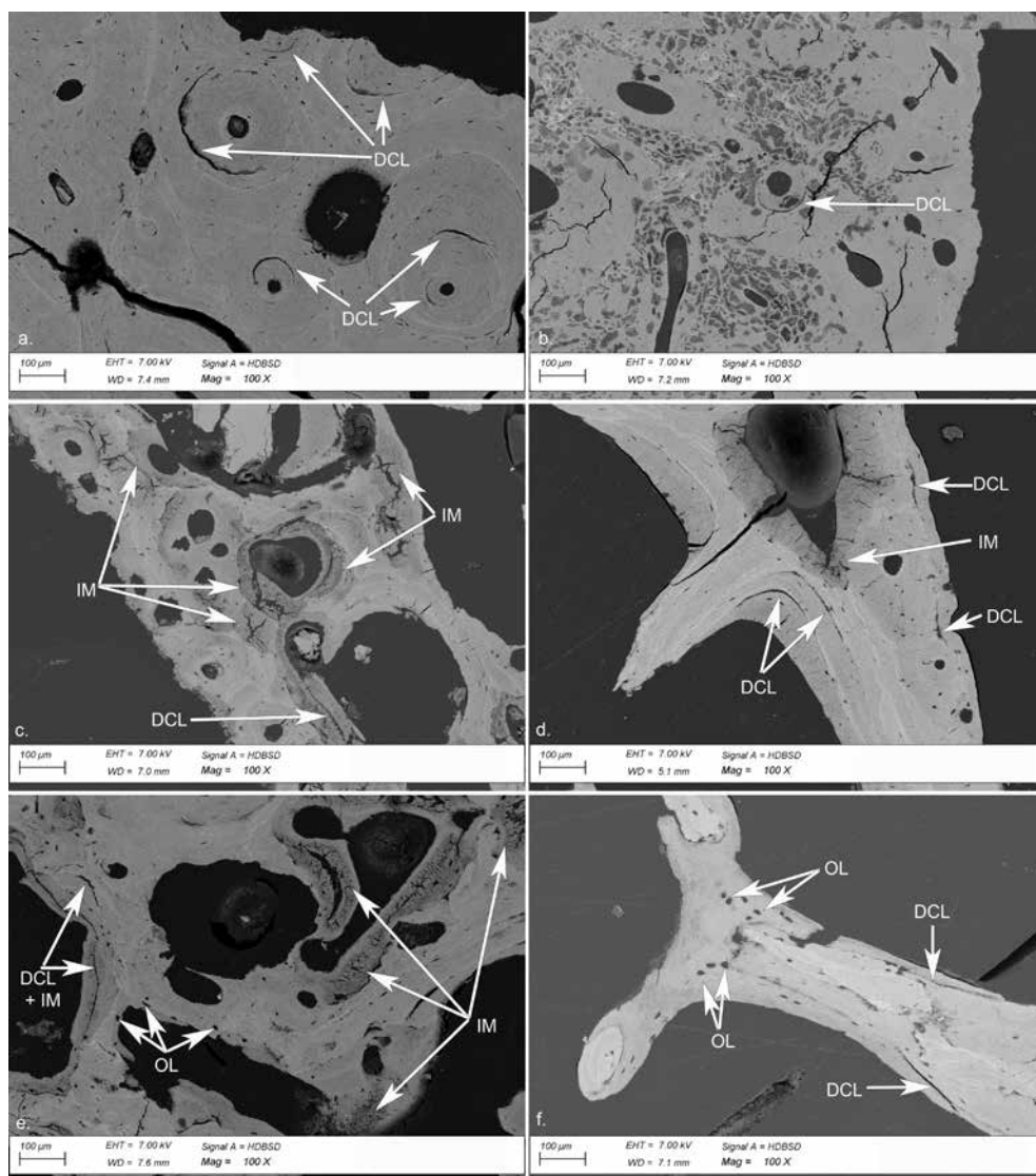
Figure 4. Composite figure of BSE-SEM images of the femoral, costal and vertebral bone samples taken from Individual 2 (MeB S2034 V138) (a., c. and e.) and Individual 3 (MeB S2037 V148) (b., d. and f.). Defective cement lines (DCL) are visible in all the sections. Note the difference in abundance of mineralization defects when comparing the femoral (a. and b.) to the costal (c. and d.) and vertebral (e. and f.) samples. Layers and/or islands of incomplete mineralization (IM) and enlarged osteocyte lacunae (OL) were mainly observed in the costal and vertebral samples. Also note the similarity in appearance of the histological features when compared with light microscopy (Figure 6). (See the Appendix online for more detailed versions of the pictures included).
