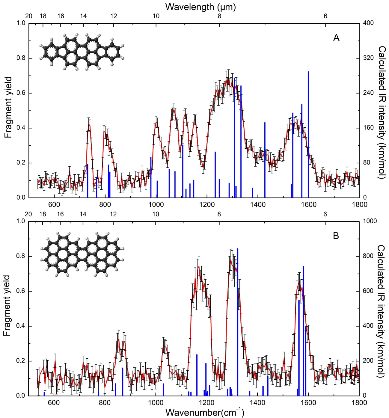
Figure 2. Measured IRMPD spectrum of gas-phase \text{DIP}^+ (upper plot) and \text{DC}^+ (lower plot). The computed vibrational peak positions scaled to correct for anharmonicities are represented by vertical bars.
