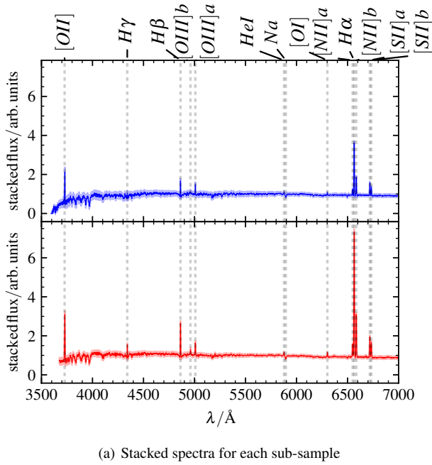
Figure 14. The median-stacked rest-frame spectra of the WISE-blue (blue) and WISE-red (red) sub-samples (left) and their locations on the MIRDD (right). The spectra were blueshifted to their rest frame and interpolated to a common wavelength grid between 3500Å and 8000Å. Each spectrum was normalised based on the median interpolated flux between 5450 and 5550Å. The 1\sigma uncertainties in the median spectra are shown as light shaded regions around the median. The MIRDD is the same as in Figure 2 with the binned q_{150\text{MHz}}^{\text{LOFAR}} taken from Figure 11 overlaid. Blue and red boxes indicate the boundaries for the WISE-blue and WISE-red sub-samples respectively.
