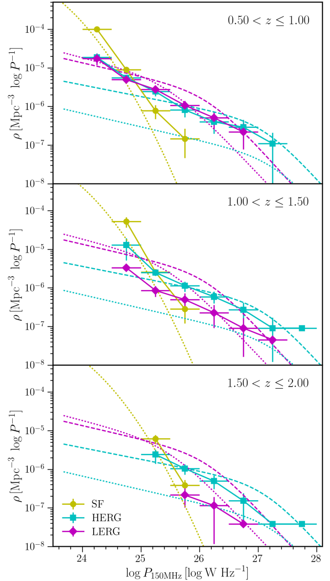
Figure 15. The radio LFs for our three intermediate redshift samples, separated into SF galaxies, HERGs and LERGs. For comparison and as a guide for the eye, the z < 0.3 (dotted) and 0.5 < z < 1.0 (dashed) HERG and LERG LFs fitted by B14 are shown in all panels. We also show the simple model SF LFs from Novak et al. (2017) at each redshift interval.
