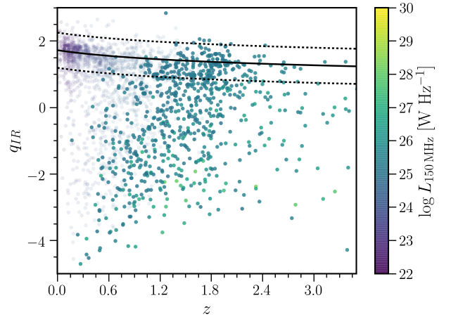
Figure 8. FIR-radio correlation, q_{IR} , computed from the IR luminosities, L_{IR} , integrated from the AGNFITTER cold dust component. The solid and dashed lines show the q_{IR} = 1.72(1+z)^{-0.22} ( \sigma = 0.529 ) FIR-radio correlation from Calistro Rivera et al. (2017). The larger points show the radio sources with P_{150\text{MHz}} \geq 10^{25} \text{ W Hz}^{-1} .
