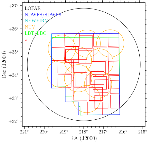
Figure 1. Coverage diagram for the Boötes field. The black circle shows the LOFAR 150-MHz coverage. The blue polygon shows the main I -selected psf-matched catalogue region, which is covered completely by both the NDWFS ( B_W R I K ) and SDWFS (3.6, 4.5, 5.8, and 8.0 \mu\text{m} ). It covers a total of 9.2 \text{deg}^2 , when regions contaminated by bright stars are excluded. The red squares show the z Boötes coverage, which has some gaps. The orange circles show the GALEX NUV coverage. There is a small area not covered by the NEWFIRM survey ( J , H , and K_s , shown in cyan) and the LBT/LBC survey ( U_{\text{spec}} , and Y , shown in light green).
