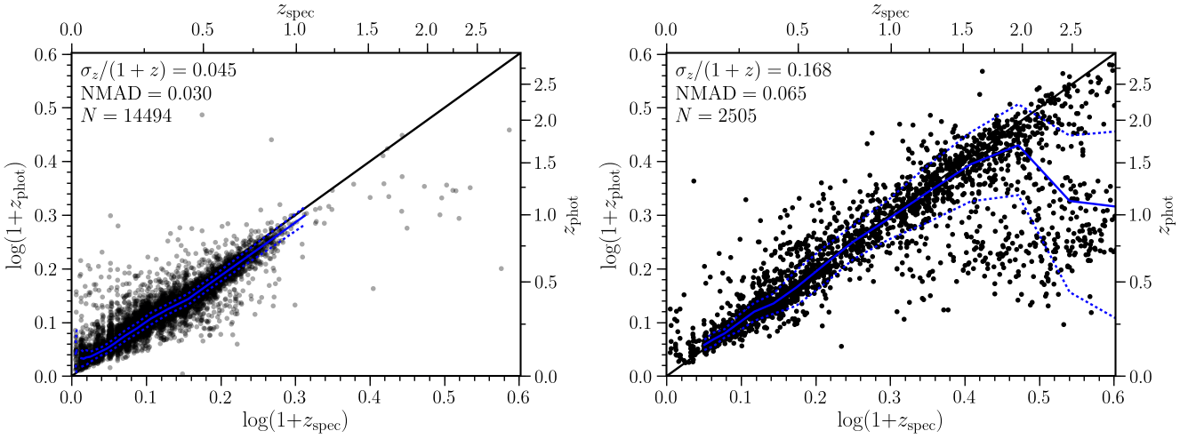
Figure 2. Photometric redshifts from the Boötes I -selected catalogue vs. spectroscopic redshifts from the AGES catalogue. Left Only galaxies not indicated as AGN in the AGES catalogue are plotted. Right Sources indicated to be AGN by the AGES SED fitting. The solid and dotted blue curves show respectively the median and rms dispersion of \delta z = (z_{\text{phot}} - z_{\text{spec}})/(1 + z_{\text{spec}}) , within 11 logarithmic-spaced bins across the spectroscopic redshift range.
