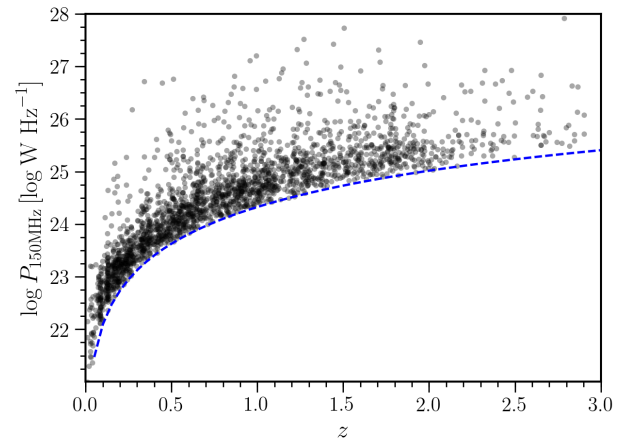
Figure 4. Distribution in the radio power vs. redshift plane of the matched radio-optical sources. The dashed blue line shows the radio power corresponding to a flux density limit of 0.5 \text{ mJy beam}^{-1} .
