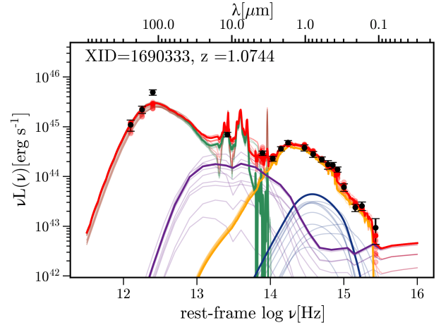
Figure 6. Example AGNFITTER SED fit showing the total model SEDs in red, and the AGN torus (purple), starburst (green), galaxy (yellow) and blue bump (blue) components. Ten realisations from the model parameters' posterior probability distributions are plotted giving an indication of the uncertainties in the fitted components. The red points show the total SEDs integrated across the filter bandpasses and the black points with error bars show the observed luminosities.
