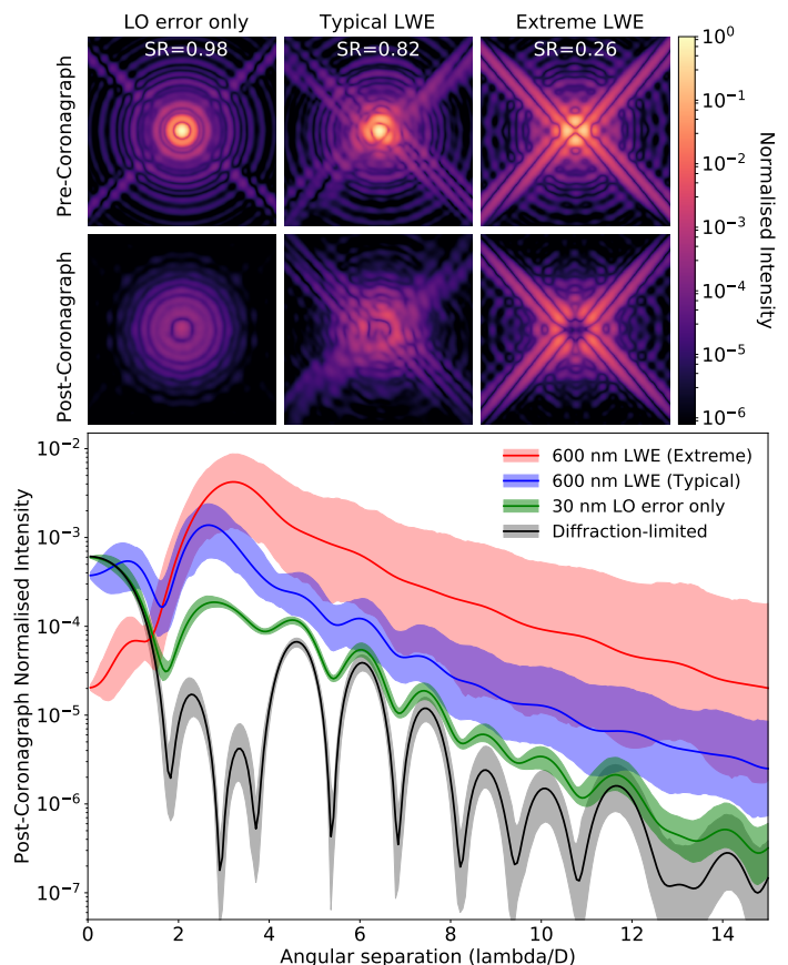
Fig. 2. Simulated performance of the SPHERE APLC in the presence of various LWE models and low-order wavefront error, for an observing wavelength of 1.536\ \mu\text{m} . Left image column: LWE-free PSFs containing only 30 nm RMS of low-order aberrations with a 1/f^2 spatial power spectrum, incoherently averaged over 100 random realisations. Centre column: a typical three-lobed LWE model (600 nm PVE) identical to Fig. 1. Right column: an extreme LWE with wavefront similar to a four-quadrant phase mask pattern (600 nm piston on two opposite VLT pupil quadrants). Top image row: non-coronagraphic PSFs, including image Strehl ratio with respect to the diffraction-limited case. Bottom image row: Corresponding on-axis coronagraphic PSFs. Main figure panel: Radial average contrast curves of each post-APLC PSF, with shading denoting the 1\sigma upper and lower bounds on azimuthal variation. Diffraction-limited performance in the absence of all aberration is shown by the black curve for comparison purposes.
