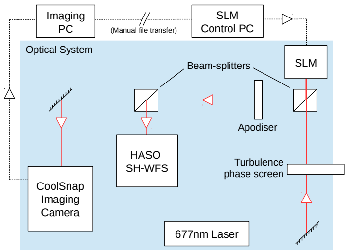
Fig. 3. Schematic of the MITHIC bench configuration used for this investigation. The spatial light modulator (SLM) is placed in a face-on reflective configuration via a double pass through a beam-splitter. Images taken via the CoolSnap camera GUI were manually transferred from the imaging PC to the SLM control PC via a separate LAM server, before performing F&F wavefront reconstruction as described in Sect. 2.2 and applying the new wavefront commands on the SLM via a custom GUI. Each closed-loop iteration of F&F typically took between 30 s and a minute to complete, of which the F&F code runtime was a negligible fraction. The HASO SH-WFS was used only for the pre-compensation of MITHIC bench alignment errors and was not operated during F&F closed-loop tests. The turbulence phase screen was aligned either on the static LWE pattern or a clear aperture, and was not used to simulate dynamical turbulence.
