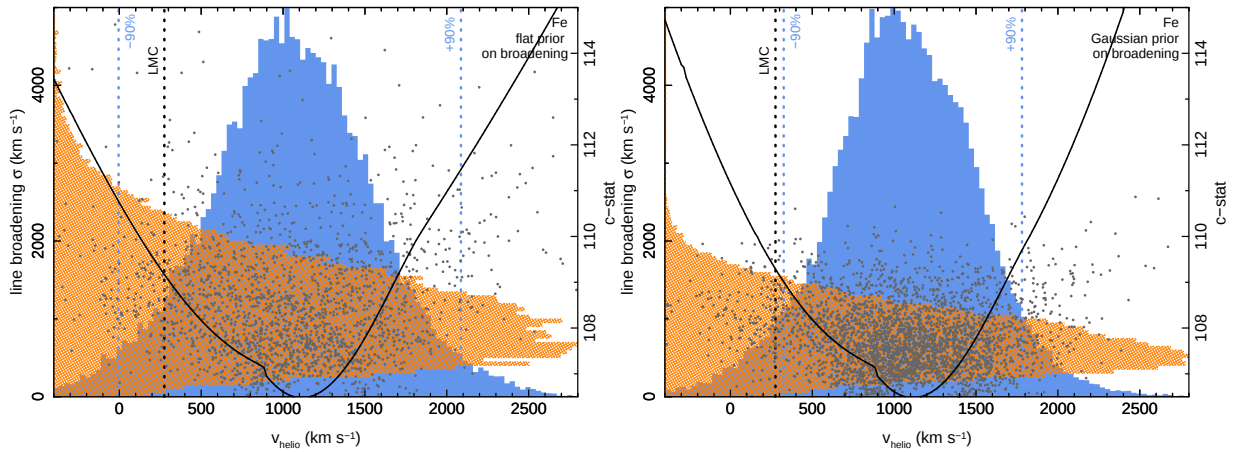
Fig. 7. Posterior probability distributions of the vrnei model broadening width (orange) and velocity (blue) from the Fe K region fitting including line broadening. Notations are the same as in figure 6. The left panel shows results with flat prior on the line width, while the right panel shows results imposing a Gaussian prior with 1-\sigma width of 1000 \text{ km s}^{-1} . Both velocity distributions trace the cstat minimization well. The flat prior produces a broader posterior distribution.
