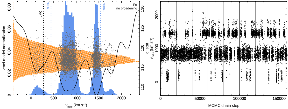
Fig. 6. (left) Posterior probability distributions of the vrnei model normalization (orange) and velocity (blue) from the Fe K region fitting without broadening, calculated from the MCMC analysis as described in the text. Points show sample MCMC chain steps, indicating that there is no correlation between the two parameters. The black line shows the cstat value from fit statistic minimization, as a function of best-fit velocity. One peak of the MCMC velocity distribution coincides with the best-fit velocity distribution, and other local peaks coincide with local cstat minima, indicating both maximum likelihood methods produce the same result. The dotted lines delineate the central 90% credible interval and note the local LMC velocity. (right) MCMC chain values for the Fe K velocity plotted against chain step, showing that the long-term variations of each chain are well-behaved and the posterior distribution is well-sampled. Vertical lines differentiate the eight individual 20,000-step simulation chains. Steps within chains are in time order with one out of every ten steps shown for clarity.
