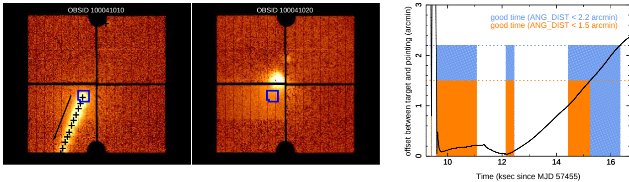
Fig. 1. (Left) SXI images in detector coordinates showing the two OBSIDs used in the SXI analysis. The blue square shows the SXS FoV. The arrow in the left panel shows the direction N132D drifted in the focal plane during that OBSID, with black crosses marking the source center in intervals of one hour. N132D was in the SXS FoV for only 3.7 ks of OBSID 100041010, and for none of OBSID 100041020. The remnant was still visible in SXI due to that detector's larger FoV. (Right) Attitude of Hitomi during the first 7 ks of OBSID 100041010. The solid line shows \text{ANG\_DIST} , the angular distance in arcmin between the intended pointing and the actual pointing. Orange bins show the good time intervals of the default data filtering, which requires \text{ANG\_DIST} < 1.5 . Blue bins show the additional \sim 43\% of time added by relaxing this criterion to 2.2 . Blank times are excluded because of Earth occultation or South Atlantic Anomaly passage.
