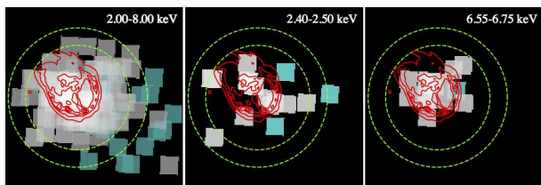
Fig. 2. Images of the SXS showing individual counts as a pixel on the sky. Blue boxes are counts included after relaxing the angular distance criterion. The red contours trace the Chandra emission, and the green circles show radii of 1.5 and 2.0 from the Chandra peak. The counts in Fe K (right) correspond well to the remnant extent, while some of the counts in the other bands are outside the bounds of the remnant.
