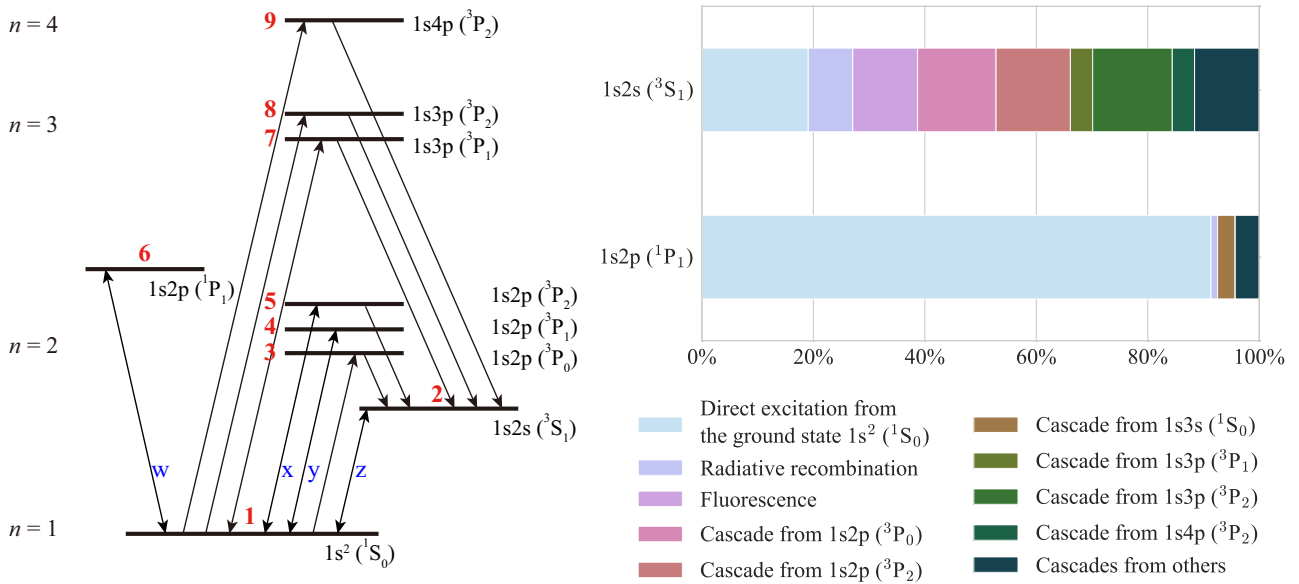
Fig. 3. (left) Grotrian diagram of the dominant Fe xxv levels to the triplet formation. Red numbers are used in table 3. Blue labels show transitions corresponding to the individual lines of the triplet. The 1s2s ( 1 S 0 ) level is not shown here, as it does not contribute to line production but to continuum emission via the two-photon decay (e.g., Nussbaumer & Schmutz 1984). (right) Relative contributions to the formations of 1s2s ( 3 S 1 ) and 1s2p ( 1 P 1 ) levels (upper levels of z and w, respectively).
