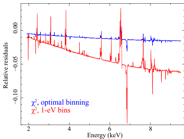
Fig. 19. Relative differences between a \chi^2 fit and a C-statistic fit (blue curve) for the baseline model. The red curve shows the same but with 1 eV bins instead of optimal binning.
