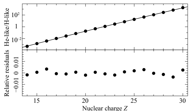
Fig. 10. (upper) He-like to H-like ion ratio as a function of nuclear charge Z for a 4-keV plasma. The solid line shows a polynomial fit in logarithm space. (lower) Relative residuals of a polynomial fit.
