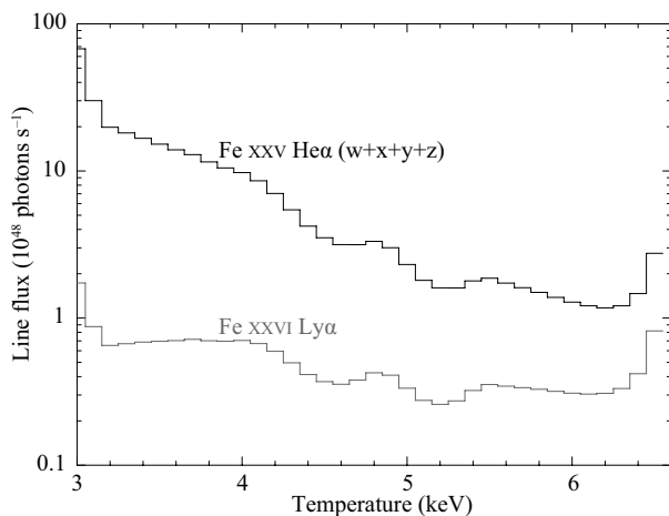
Fig. 14. The predicted distribution of the line flux of the main n=1-2 transitions of Fe XXV and Fe XXVI within the Hitomi SXS FOV.
