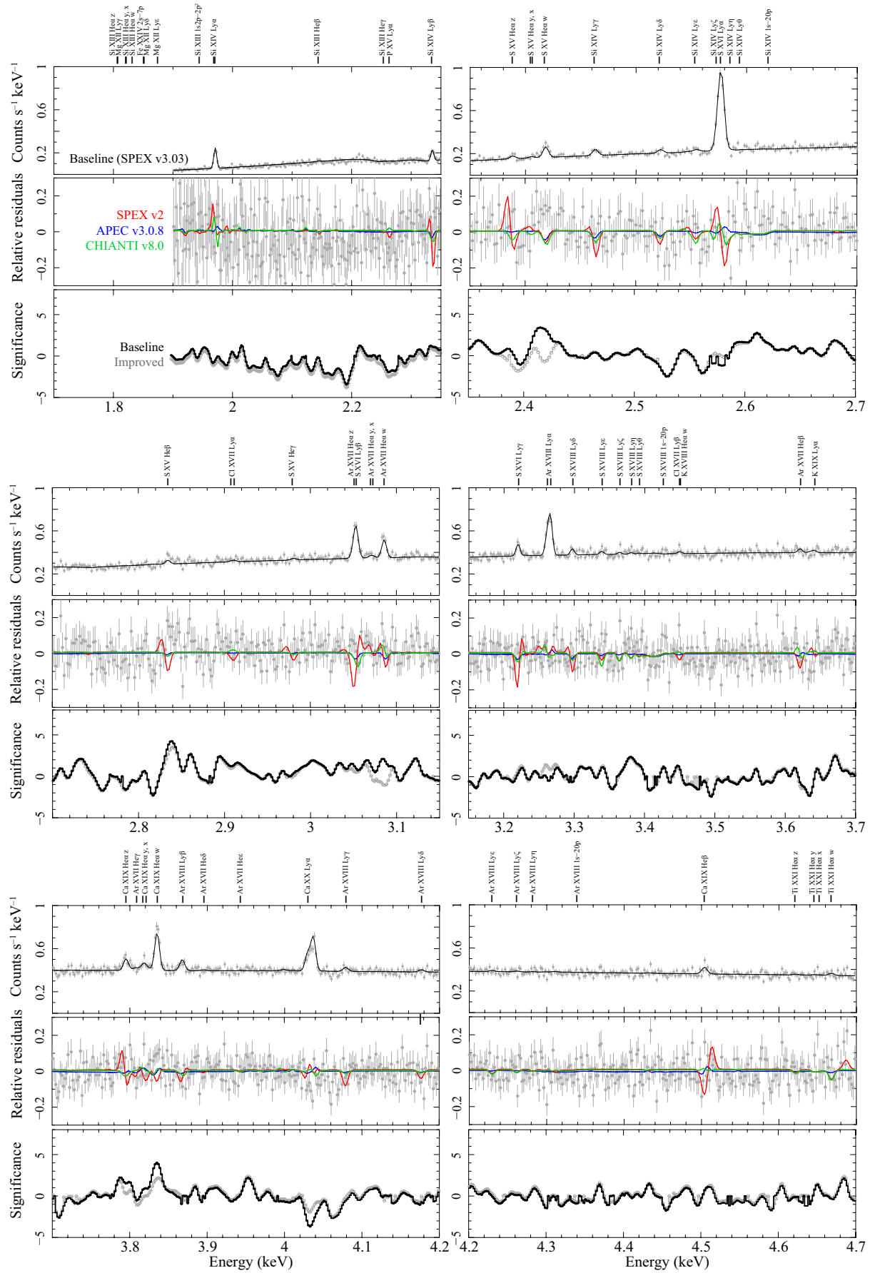
Fig. 23. The SXS spectrum of the Perseus cluster in 1.9–4.7 keV fitted with different models. Panels in each subfigure show (upper) fit to the data with the baseline model, (middle) relative difference between the baseline model and the best-fit models with APEC v3.0.8 in blue, SPEX v2 in red, and CHIANTI v8.0 in green, and (lower) significances in \sigma of an additional line model at each energy on top of the baseline model in black and improved model in grey.
