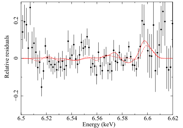
Fig. 11. Residuals of the baseline model near the He-like 1s-2p transitions. The dotted curve shows the predicted model change when instead of Doppler profiles Voigt profiles are chosen, but without altering the parameters of the baseline model. The solid curve shows the same but after refitting the spectrum.
