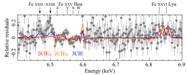
Fig. 16. Residuals of the baseline fitting in the Fe band. The red, orange, and blue curves show the changes by the 2CIE A , 2CIE B , and 3CIE models, respectively. The black arrows indicate the redshifted energies of Fe XXII and Fe XXIII DR line complex.
