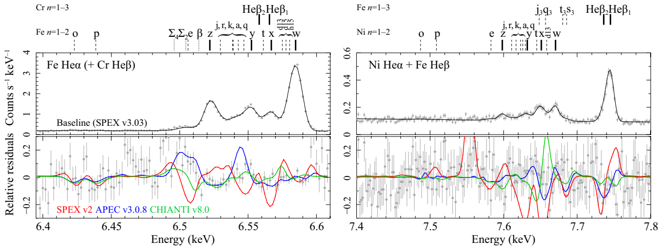
Fig. 1. The Hitomi SXS spectrum in the Fe (left) and Ni (right) He \alpha bands with the best-fit baseline model in the upper panels, and the residuals in the lower panels. Also shown in the lower panels are the relative difference between the baseline model and the best-fit models with various other plasma codes (SPEX v2 in red, APEC v3.0.8 in blue, and CHIANTI v8.0 in green). Solid bars above the upper panels show energies of the main He \alpha and He \beta lines, while dashed and dotted ones are respectively of the Li-like and Be-like satellite lines. For the full-band results and line notations see appendices 4 and 5, respectively.
