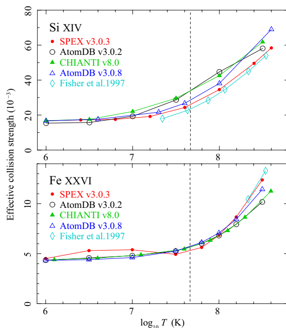
Fig. 2. Comparisons of effective collision strength as a function of balance temperature. The Ly \alpha 1 and Ly \alpha 2 transitions are combined. The vertical dashed lines mark a temperature of 4 keV.
