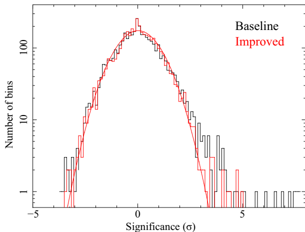
Fig. 20. Diagrams showing the significance of an additional line model, on the top of the best-fit baseline model (black) and improved model (red), with the central energy moving across the entire band. The red curve shows a \sigma = 1 Gaussian function that fits the diagram of the improved model.
