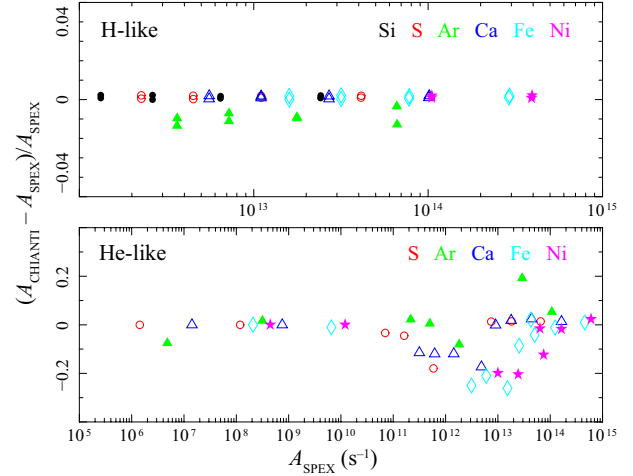
Fig. 7. Same as figure 6, but for comparison between SPEX v3.03 and CHIANTI v8.0.
