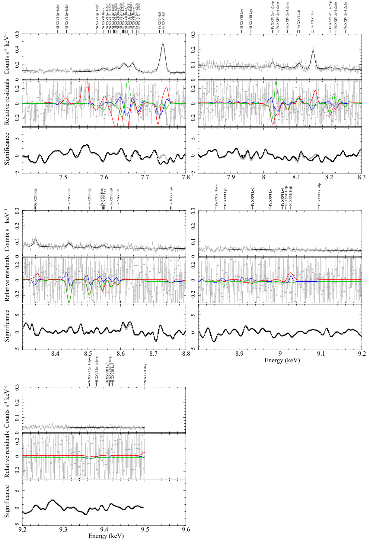
Fig. 25. The same as figure 23, but in 7.4–9.5 keV.
