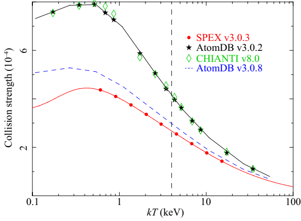
Fig. 4. Comparison of the effective collision strength from the ground to 1s2s ( ^3S_1 ) state. The vertical line shows a temperature of 4 keV.
