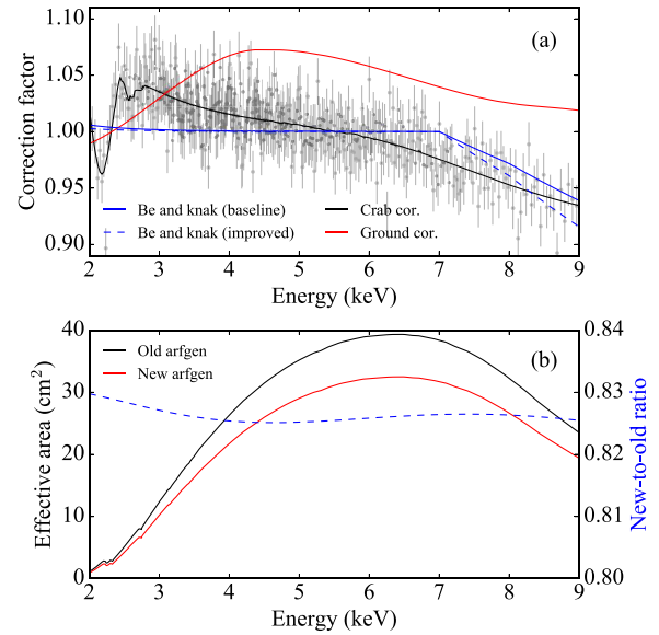
Fig. 22. (a) A comparison of effective area correction factors: the original correction (blue) for each of the baseline and improved models respectively in solid and dashed curves, the on-ground calibration correction (red), and the Crab correction (black) derived by smoothing the SXS-to-canonical ratio (grey crosses: private communication with M. Tsujimoto, 2017). For the Crab analysis, the high-primary as well as mid-primary grade events are used. (b) Effective area with the old and the new arfgen in black and red, respectively, as well as the ratio of the two calculations with the dashed blue curve.
