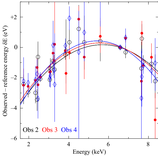
Fig. 21. The differences between measured and reference energies of the brightest lines (see table 8 for details). The curves show the best-fit parabolic functions of the three observations.
