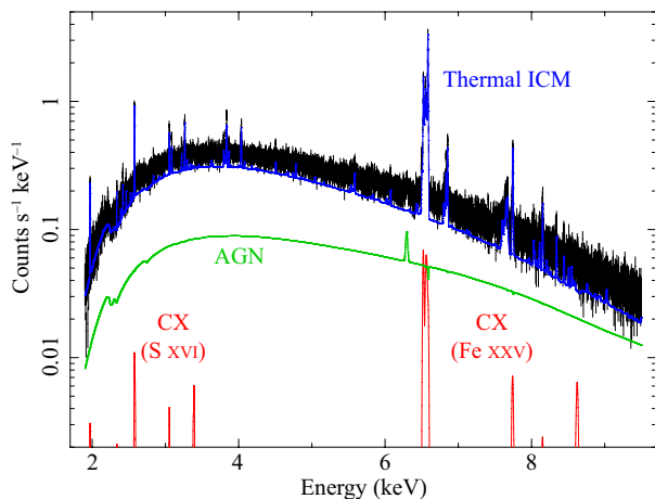
Fig. 17. The best-fit result with the CX emission. Each X-ray emission component is shown: thermal ICM in blue, AGN in green, and CX in red.
