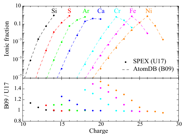
Fig. 9. (upper) Ionic fraction of a 4-keV CIE plasma in SPEX v3.03 (U17: dots) and APEC v3.0.8 (B09: curves). (lower) Ratios between the two.
