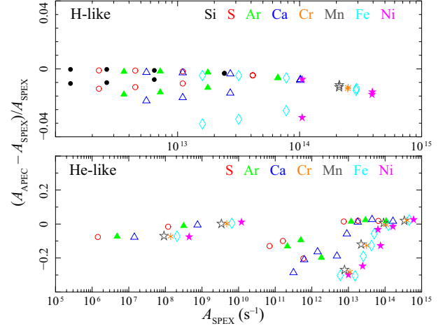
Fig. 6. The differences of Einstein A values of the strongest transitions (table 10) in SPEX v3.03 and AtomDB v3.0.8 for the H-like (upper) and He-like (lower) ions. The upper states are in the range of n = 2-5 for H-like and 2-4 for He-like ions.
