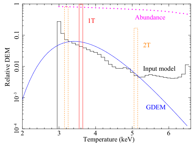
Fig. 13. The predicted DEM profile of the Perseus cluster within the FOV of the Hitomi SXS (black histogram) and the corresponding average abundance profile (relative to the proto-solar values of Lodders & Palme 2009; magenta dots). The best-fit isothermal (1T) and two-temperature (2T) models to this DEM are shown with the red and orange histograms, respectively, and the best-fit GDEM model with the blue curve.
