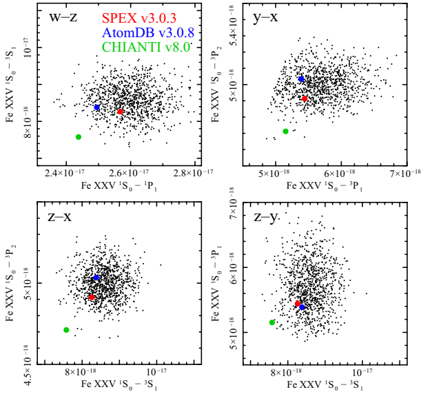
Fig. 5. Monte-Carlo simulations on the four Fe XXV He \alpha lines. The SPEX, AtomDB, and CHIANTI values are shown in red, blue, and green, respectively. The line intensities are given in the unit of photon \text{cm}^{-3} \text{s}^{-1} .
