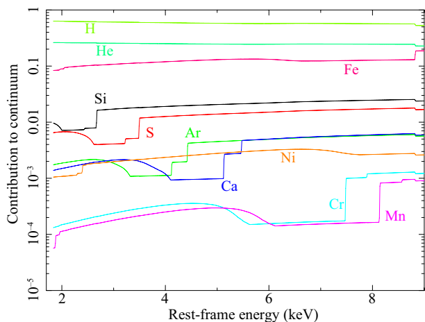
Fig. 12. Relative contribution of the different elements to the continuum emission of the main thermal component in the Perseus cluster.
