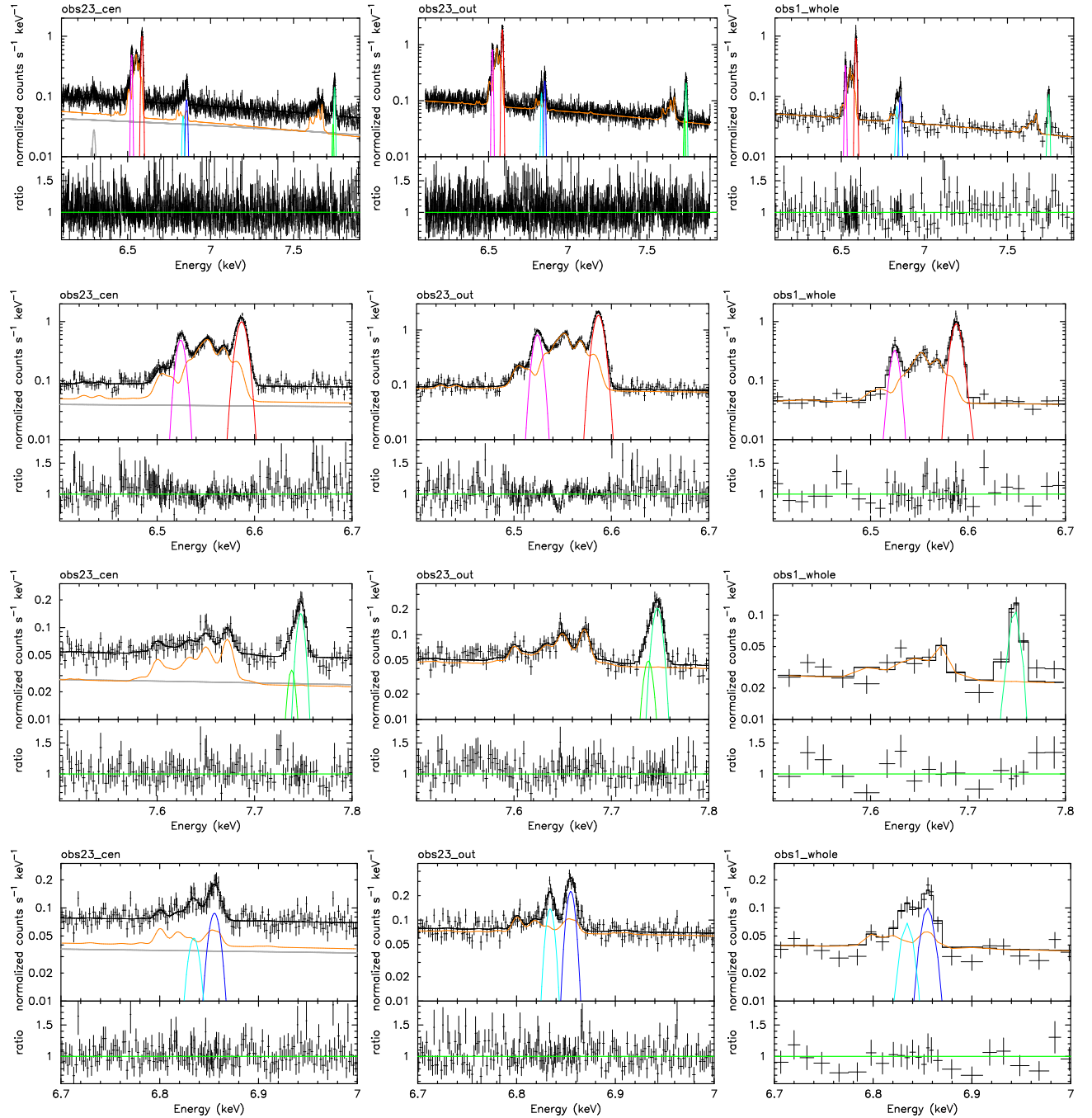
Fig. 2. The observed Hitomi spectra extracted from the obs23_cen, obs23_out and obs1_whole regions shown in figure 1, and binned for display purposes. Top panels show the resultant spectral fits in 6.1–7.9 keV band, while the second, third and fourth rows show the energy range of the He \alpha complex, and He \beta , and Ly \alpha lines in 6.4–6.7, 7.5–7.8, and 6.7–7 keV, respectively. The spectra obtained with the Hitomi SXS are shown in black; light gray lines show the emission from the AGN. Orange lines indicate the “modified” bvapec model, in which the strongest lines have been deleted. The Fe xxv He \alpha forbidden and resonance, He \beta_{1,2} , and Fe xxvi Ly \alpha_{1,2} are shown in magenta, red, green, light green, blue and cyan lines, respectively. The lower panels show the fit residuals in units of ratio.
