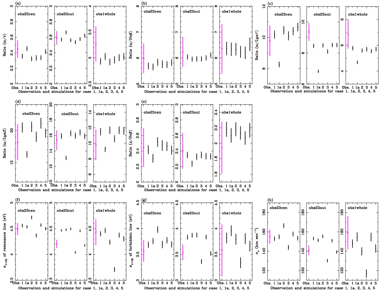
Fig. 10. (a)–(e): Comparisons of line ratios of the Fe He \alpha resonance (w) to forbidden (z), He \beta , and Ly \alpha_{1,2} , and the Fe He \alpha w to He \beta between observation (magenta, noted as Obs.) and simulations with RS for case 1, 1a, 2, 3, 4, and 5. (f)–(g): Same as line widths of the w and z. (h): Same as the derived \sigma_v from the mock spectra.
