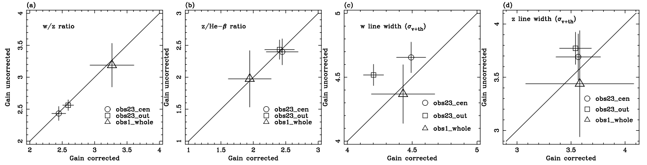
Fig. 6. Scattering plots between the gain corrected and uncorrected data for (a) the w/z line ratio, (b) the z/\text{He}\beta line ratio, (c) w line width ( \sigma_{v+th} ) and (d) z line width ( \sigma_{v+th} ). Open circles, squares, and triangles correspond to the measurements in the obs23_cen, obs23_out, and obs1_whole regions, respectively.
