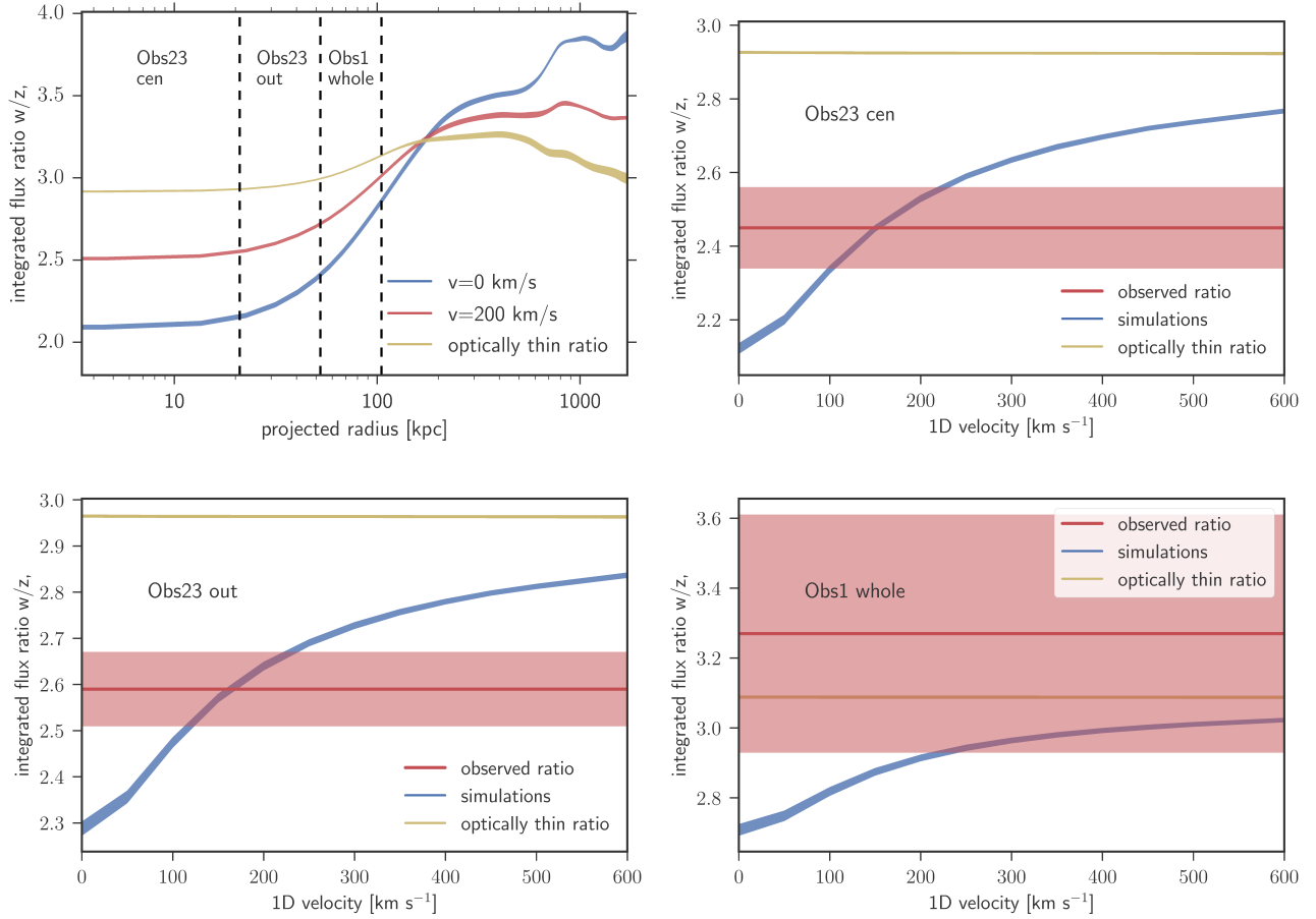
Fig. 11. Top, left: the w/z ratio as a function of projected distance from the cluster center calculated using ICMC simulations of RS assuming zero (blue) and 200 \text{ km s}^{-1} (red) velocity of gas motions along the line of sight. The optically thin line ratio is shown in yellow. All ratios are combined with the Hitomi PSF. The width of each curve reflects the 1\sigma statistical uncertainty on the deprojected thermodynamic profiles (see figure 7). The approximate locations of spectral extraction regions (obs23_cen, obs23_out, and obs1_whole) are shown with dashed lines. Top, right and bottom: integrated flux ratio over spectral extraction regions (see figure 1) as a function of line-of-sight velocity (blue); integrated optically thin line ratio vs. velocity (yellow) and the observed line ratio from the Hitomi data (red). The overlap between the red regions and blue curves provides constraints on the velocity of gas motions.
