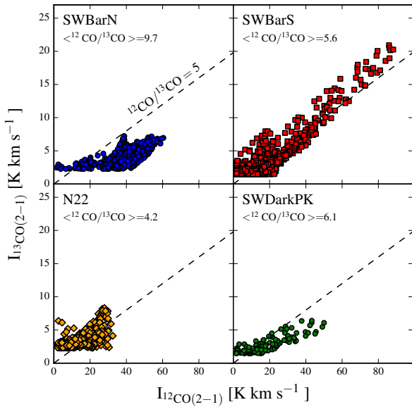
Figure 9. Ratio of integrated intensity of ^{12}\text{CO} (2 – 1) to ^{13}\text{CO} where both are detected at > 3\sigma . The average ^{12}\text{CO}/^{13}\text{CO} ( \langle^{12}\text{CO}/^{13}\text{CO}\rangle ) are listed for each region. The dashed line shows a typical ratio found in the Milky Way of ^{12}\text{CO}/^{13}\text{CO} = 5 .
