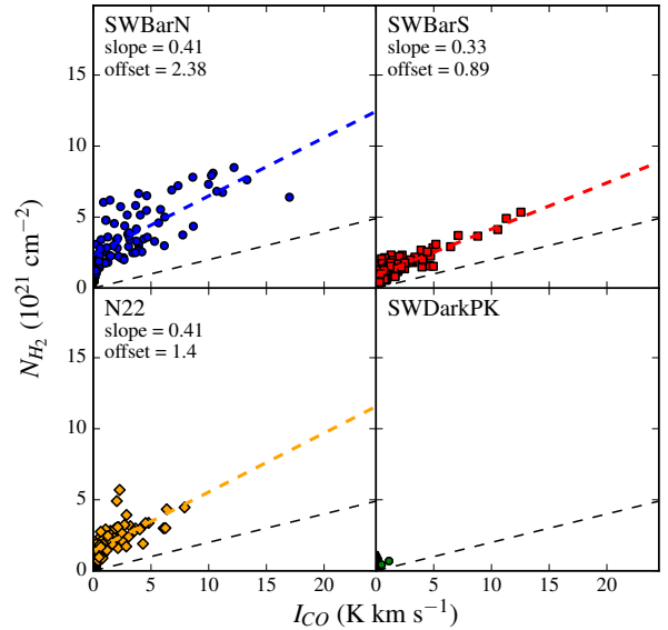
Figure 19. Relationship between I_{\text{CO}} and N_{\text{H}_2} for the ALMA regions where N_{\text{H}_2} is the combined estimate of \text{H}_2 from [C II] and from CO using the Galactic CO-to- \text{H}_2 conversion factor X_{\text{CO}} = 2 \times 10^{20} \text{ cm}^{-2} (\text{K km s}^{-1})^{-1} . The colored symbols show independent measurements detected at > 3\sigma in ^{12}\text{CO} . There is good correlation between CO and \text{H}_2 , and the slope of the relationship is X_{\text{CO}} . The thick dashed colored lines show the linear fits to the data; the steeper slopes correspond to higher values of X_{\text{CO}} . The over plotted black dashed lines shows the Galactic conversion factor ( X_{\text{CO}} ) appropriate for the Milky Way and resolved measurements (Bolatto et al. 2013).
