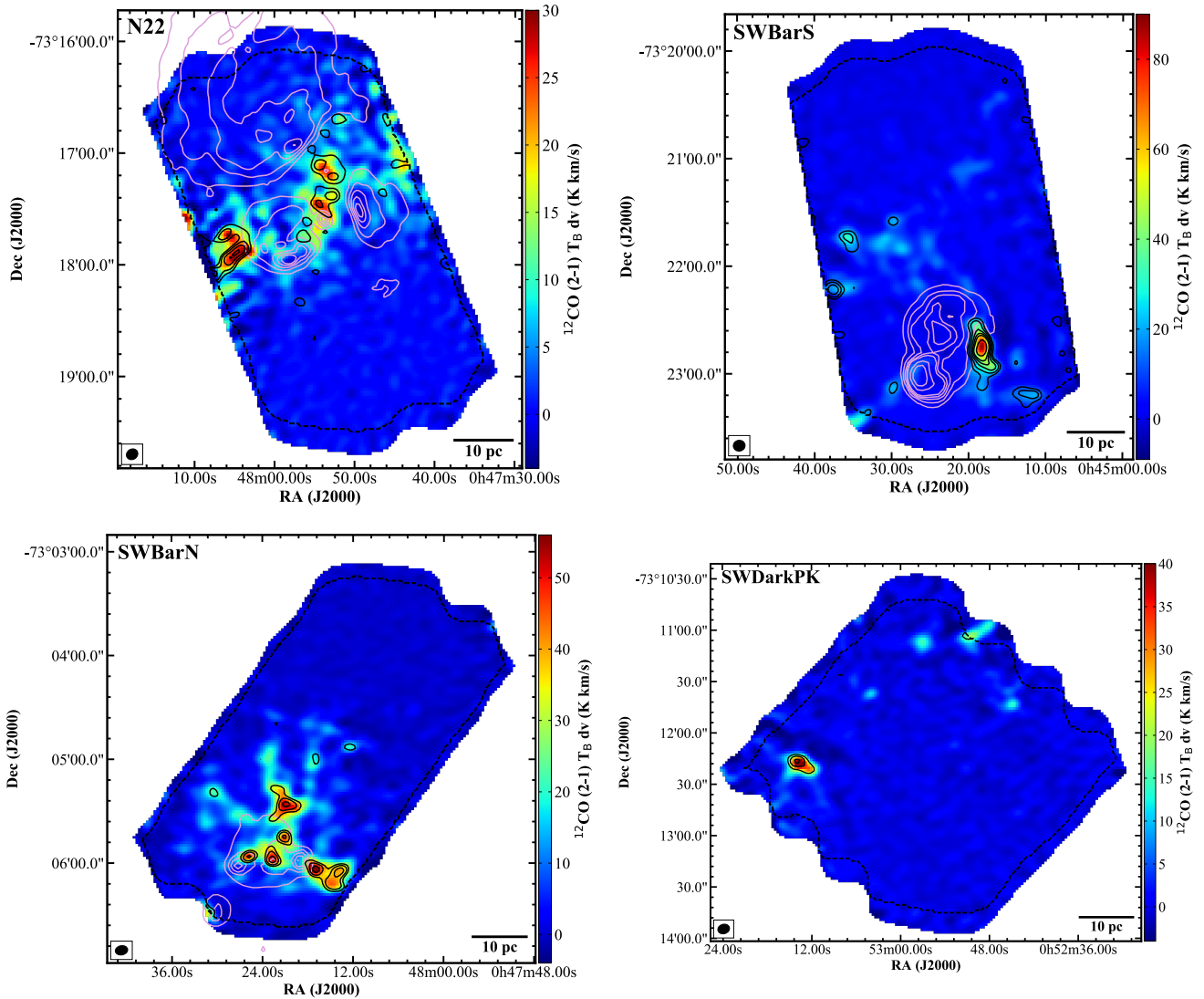
Figure 8. Integrated intensity maps of ALMA ACA+TP ^{12}\text{CO} (2–1) with black contours showing ALMA ACA ^{13}\text{CO} (2–1) at levels of 2.5, 4, 6, 8, 10, 15 \text{K km s}^{-1} and the light purple contours showing the \text{H}\alpha contours shown in Figure 1. The black dashed line shows the coverage of the ^{13}\text{CO} (2–1) image. The sensitivities of the maps are listed in Table 5.
