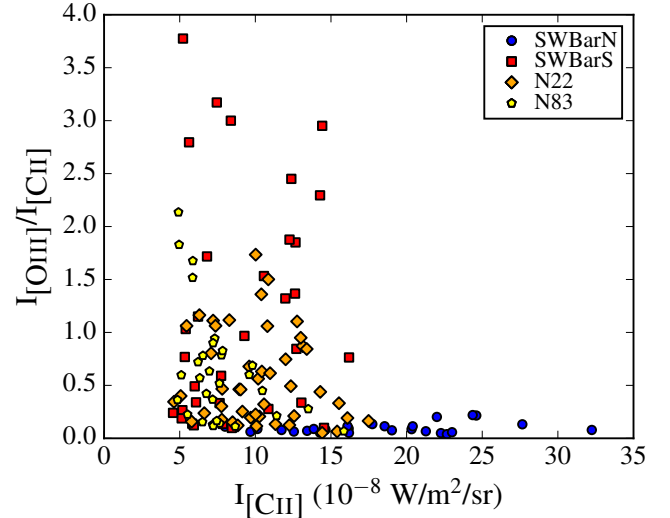
Figure 7. Ratio of integrated intensities of [O III] 88 \mu\text{m} ( I_{[\text{OIII}]} ) to [C II] ( I_{[\text{CII}]} ) as a function of the [C II] intensity where [O III] is detected at > 3\sigma for each of the regions. The [O III] maps cover the main H II regions in the HS 3 regions. We see high I_{[\text{OIII}]} / I_{[\text{CII}]} ratios in all of the regions except SWBarN where there is no large H II region and likely less ionized gas.
