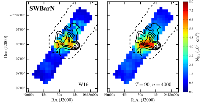
Figure 16. Images of the estimate of N_{H_2} from the [C II] emission for the SWBarN region using Method 2 using Wolfire et al. (2017, in preparation) models (left) and Method 1 with a fixed T = 90 K and n = 4000 cm^3 (right), shown at the same scale. The black contours show the estimate of N_{H_2} from ^{12}CO (using X_{CO} = 2 \times 10^{20} ) at levels of 0.4, 0.8, 1.4, and 2.4 \times 10^{21} cm^{-2} and the black dashed line shows the coverage of the ^{12}CO map. Both N_{H_2} estimates from [C II] produce similar average estimates of N_{H_2} , but the structures are different. When taking into account the local T and n using the Wolfire et al. (2017, in preparation) results, there is less H_2 needed to explain the [C II] emission at the center of the cloud (the peak of the ^{12}CO emission). The estimated N_{H_2} peaks away from the ^{12}CO peak, which is consistent with the [C II] emission tracing the CO-faint H_2 in the photodissociation region, suggesting that the H_2 estimates using the new models are more accurate.
