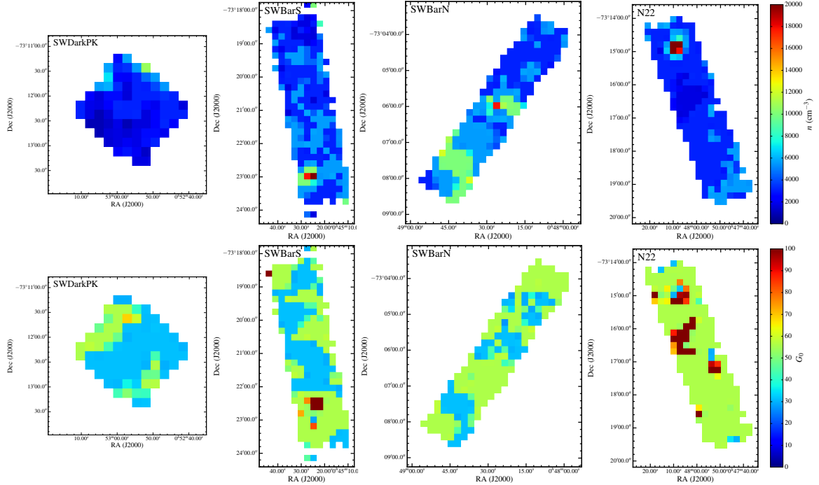
Figure 14. Density and radiation field for each of the regions with HS 3 and ALMA data, obtained from physical PDR modeling developed for the conditions in the SMC (abundances, cosmic ray rates, dust to gas ratio, etc; see Appendix A). The top row shows volume density ( n ), and the bottom row shows FUV radiation field strength ( G_0 ). If [C II] dominates the cooling, then the [C II] line intensity is proportional to G_0 . The appropriate [C II] cooling rate per H 2 molecule for each pixel is determined by taking the [C II] cooling rate appropriate for the specific value of n and then scaling it linearly by the ratio of estimated G_0 to the fiducial G_0 for diffuse gas. We then use this local [C II] cooling rate to calculate a H 2 column density and produce the final map. The benefit of this method is that it can account for the variations in density and radiation field in the [C II]-emitting gas throughout the regions. The weakness is that the gas conditions are estimated using “single component” models based on plane-parallel PDRs that do not account for complex geometries, or for distributions of n or G_0 within a spatial resolution element. This is alleviated by the fact that our physical resolution is 4 pc, thus we expect the conditions in a beam to be relatively uniform and simple “single component” models to be more applicable than they would be if applied to data on much larger scales.
