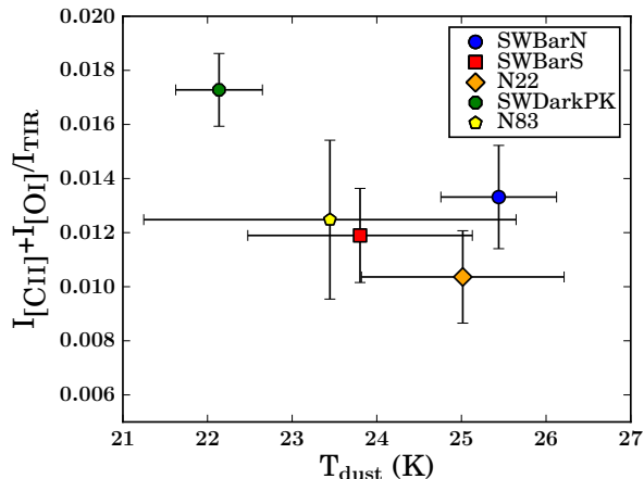
Figure 4. The mean ratios of the [C II] and [O I] intensities to the TIR, an indicator of the photoelectric heating efficiency, as a function of mean dust temperature ( T_{\text{dust}} ) from Lee et al. (2015). The error bars show 1\sigma on the mean.
