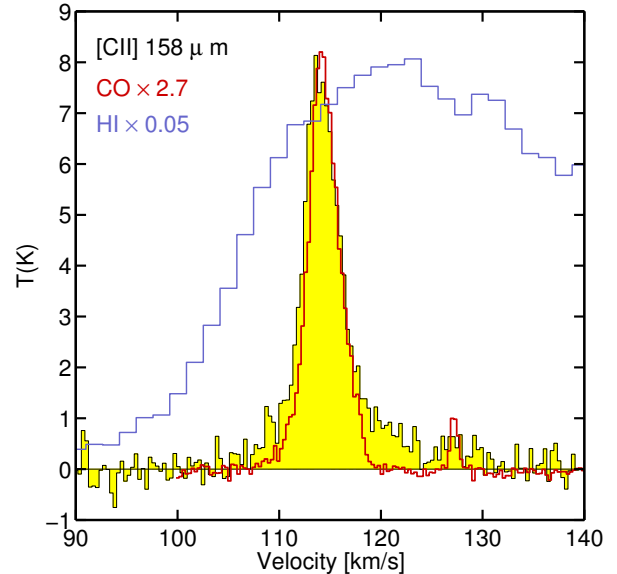
Figure 12. Spectrum of [C II] from one pointing observed with SOFIA GREAT (R. Herrera-Camus et al. 2017, in preparation; region R8) with the yellow filled histogram showing the data in 0.3 \text{ km s}^{-1} bins with scaled spectra of the ALMA ^{12}\text{CO} (2 – 1) in red and H I in purple for the same area in the SWBarN region with velocity in the LSRK reference frame. This illustrates that the velocity profile of the [C II] emission is most similar to the ^{12}\text{CO} and not the H I, suggesting that a significant fraction of the emission comes from molecular gas. It also shows that the [C II] emission profile can have wider wings at low or no ^{12}\text{CO} intensity, in this case by 5 - 10 \text{ km s}^{-1} , which makes the total extent of the [C II] profile wider (by at most \sim 50\% ) than the ^{12}\text{CO} line profile and has wider .
