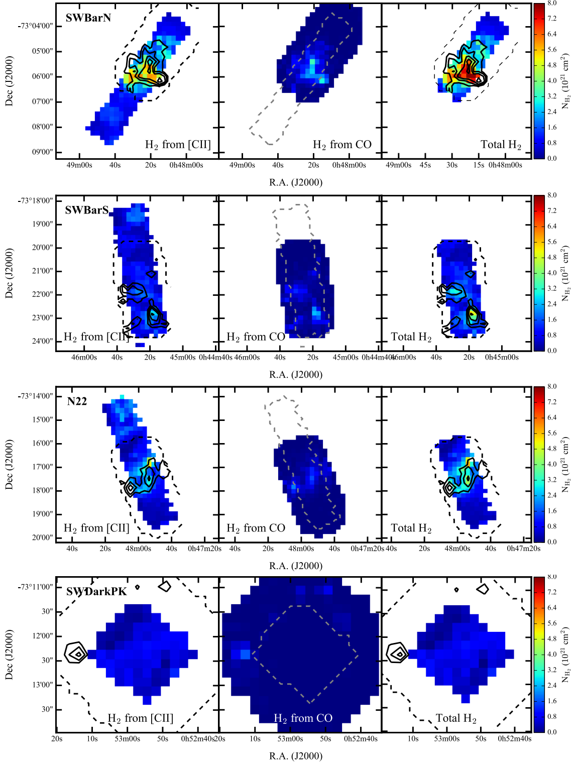
Figure 17. Images of N_{\text{H}_2} for each of the regions with Herschel and ALMA data. The images on the left shows the estimate of N_{\text{H}_2} from the [C II] emission using Method 2 (W16 n , G_0 ) described in Section 4.3.2. The middle images shows N_{\text{H}_2} traced by ^{12}\text{CO} , with the ALMA (2 – 1) converted to (1 – 0) assuming thermalized emission, and assuming a Galactic X_{\text{CO}} of 2 \times 10^{20} \text{ cm}^{-2} (\text{K km s}^{-1})^{-1} . The images on the right show total N_{\text{H}_2} found by combining the estimate from [C II] with the estimate from ^{12}\text{CO} . The black contours show the estimate of N_{\text{H}_2} from ^{12}\text{CO} at levels of 0.4, 0.8, 1.4, \text{ and } 2.4 \times 10^{21} \text{ cm}^{-2} and the black dashed line shows the coverage of the ^{12}\text{CO} map. The grey dashed line shows the \text{HS}^3 ([C II] and [O I]) coverage. All maps are shown at the same color scale.
