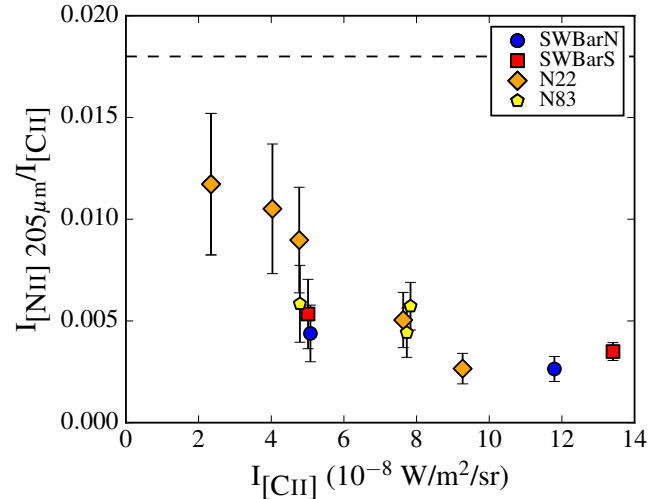
Figure 6. Ratio of integrated intensities of [N II] 205 \mu\text{m} ( I_{[\text{NII}] 205 \mu\text{m}} ) to [C II] ( I_{[\text{CII}]} ) as a function of the [C II] intensity for FTS bolometer measurement of [N II] 205 \mu\text{m} that is > 3\sigma for each of the regions. The error bars show the 1\sigma uncertainty on the line ratio, which is dominated by the uncertainty in the [N II] 205 \mu\text{m} flux (the uncertainty in I_{[\text{CII}]} is smaller than the symbols). The FTS pointings for each of the regions targeted the star-forming peak, which tends to coincide with the peak CO emission. The ratios are low and naturally peak towards higher values at lower [C II] intensities. The black dashed line shows the lowest observed ratio of [N II] 205 \mu\text{m} /[C II] \sim 0.018 in the KINGFISH sample ( Croxall et al. 2017 ).
