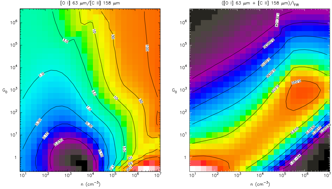
Figure A1. New SMC PDR model contour plots for the [O I] 63 \mu\text{m} /[C II] 158 \mu\text{m} (left) and ([\text{O I}] 63 \mu\text{m} + [\text{C II}] 158 \mu\text{m})/\text{FIR} ratios as a function of n and G_0 .
