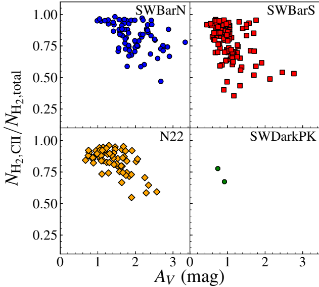
Figure 18. Relationship between the ratio of N_{\text{H}_2, [\text{CII}]} to N_{\text{H}_2, \text{total}} for the ALMA regions where N_{\text{H}_2, \text{total}} is the combined estimate of \text{H}_2 from [C II] and \text{H}_2 from CO, the latter using a Galactic CO-to- \text{H}_2 conversion factor X_{\text{CO}} = 2 \times 10^{20} \text{ cm}^{-2} (\text{K km s}^{-1})^{-1} . The colored symbols show independent measurements with I_{12\text{CO}} > 3\sigma .
