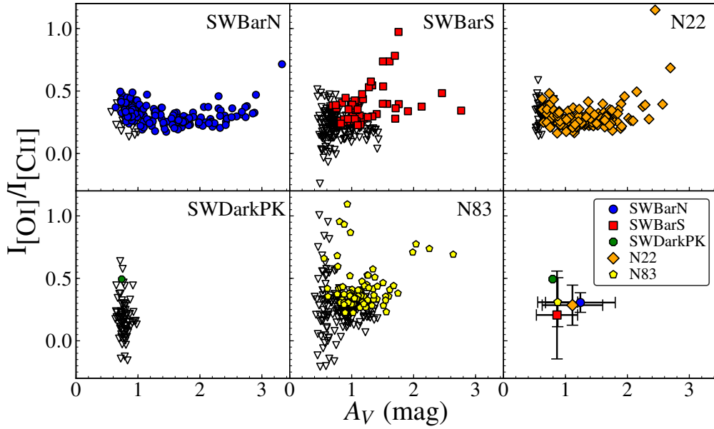
Figure 2. The ratio of the integrated intensity of [O I] to that of [C II] as a function of A_V for the HS 3 regions. The colored symbols show independent measurements detected at > 3\sigma in both [O I] and [C II] with the downward pointing triangles indicating upper limits (where I_{[\text{O I}]} < 3\sigma ). The bottom right panel shows the average values with the error bars showing 1\sigma on mean for each of the regions except for SWDarkPK, for which we show the one measurement > 3\sigma . The mean line ratios were calculated to include the upper limits (“left-censored” data) using the cenfit routine in the R package NADA (Lee 2017; Helsel 2005). The [O I]/[C II] ratio is mostly constant across the regions, independent of A_V , and has a typical value of \sim 0.3 .
