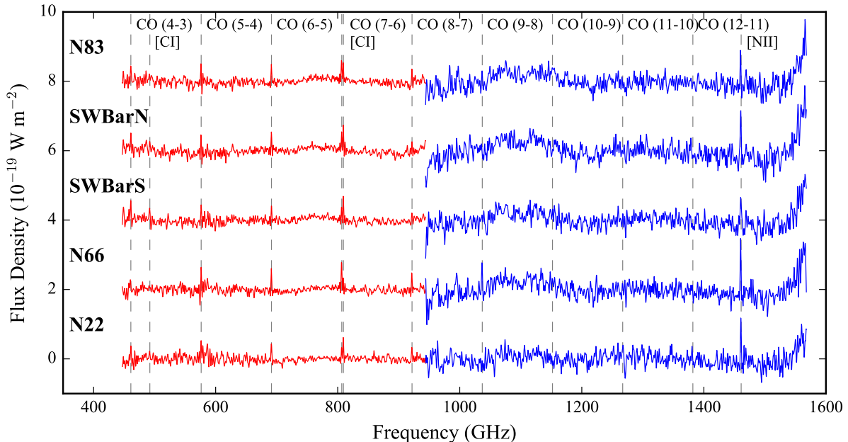
Figure 5. FTS SLW (red) and SSW (blue) spectra averaged over all the bolometers for HS 3 regions SWBarN, SWBarS, N22, and N83, plus N66 (the target of PACS observations from the Herschel GTKP SHINING project) with each spectra being offset by 2 \times 10^{-19} \text{ W m}^{-2} \text{ sr}^{-1} . The SLW and SSW spectra have a second-order polynomial fit and subtracted to remove the baseline. The grey dashed lines indicate the positions of possible spectral lines. There are no detections of the CO ladder in the SSW except for CO (9–8) in N66, which also displays CO (8–7) in the SLW, showing that gas associated with the molecular complex in this giant H II region is warm and highly excited.
