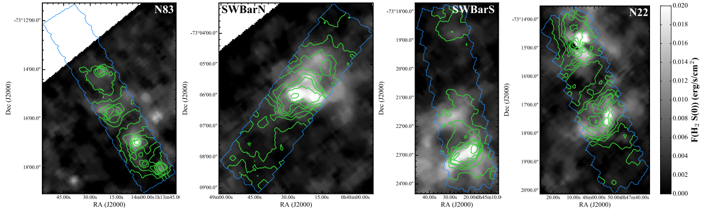
Figure 3. Images of the \text{H}_2 \text{S}(0) 28.2 \mu\text{m} line from \text{S}^4\text{MC} (Sandstrom et al. 2012) resampled to match the \text{HS}^3 [\text{C II}] images. Contours show the [\text{C II}] integrated intensity at levels of 0.3, 0.5, 0.7, 0.9, 1.2, 1.5, 2.0, 3.0 \times 10^{-7} \text{ W m}^{-2} \text{ sr}^{-1} , with the blue line showing the [\text{C II}] map coverage. The excellent correspondence between the structures provides evidence that [\text{C II}] is tracing the molecular gas in the PDRs.
