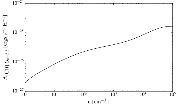
Figure 15. [C II] cooling rate ( \Lambda_{[C II]} ) as a function of density for the conditions in the SMC from Wolfire et al. (2017, in preparation) used to convert the [C II] emission to a column density of H_2 . The cooling curve is calculated assuming G_0 = 5.5 .
