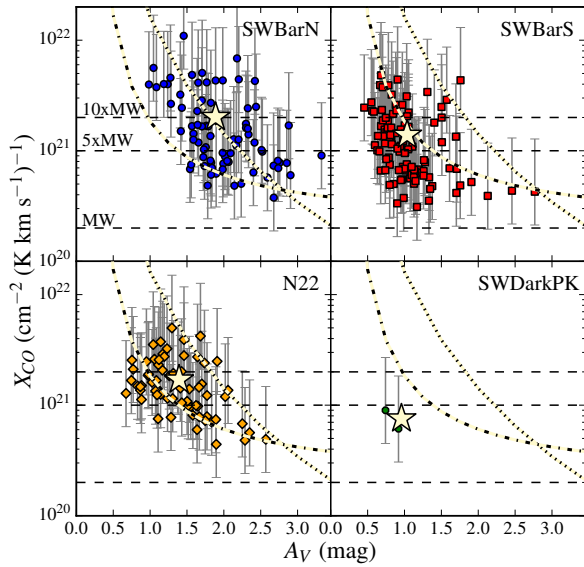
Figure 20. The CO-to-H 2 conversion factor ( X_{CO} ) as a function of A_V for the ALMA regions where the H 2 used is the combined estimate of H 2 from [C II] and H 2 from CO using a Galactic value of X_{CO} = 2 \times 10^{20} \text{ cm}^{-2} (\text{K km s}^{-1})^{-1} . The colored symbols show independent measurements detected at > 3\sigma in 12 CO with the error bars showing the factor of 2 uncertainty in N_{\text{H}_2} , with the star symbols showing the mean A_V and X_{CO} for each region. The over plotted dashed lines show scalings of the Galactic conversion factor appropriate for the Milky Way and resolved measurements (Bolatto et al. 2013). The dotted line shows the estimate of X_{CO} -based average CO luminosity, the average N_{\text{H}_2} , and the average A_V over the entire cloud for the simulations of molecular clouds by Glover & Mac Low (2011). The dash-dotted line shows similar cloud-averaged estimate of X_{CO} as a function of A_V from the PDR models from Wolfire et al. (2010) for the SMC metallicity and radiation field strength of 40 G_0 , the approximate mean radiation field found in the regions (see Section 4.3.2).
