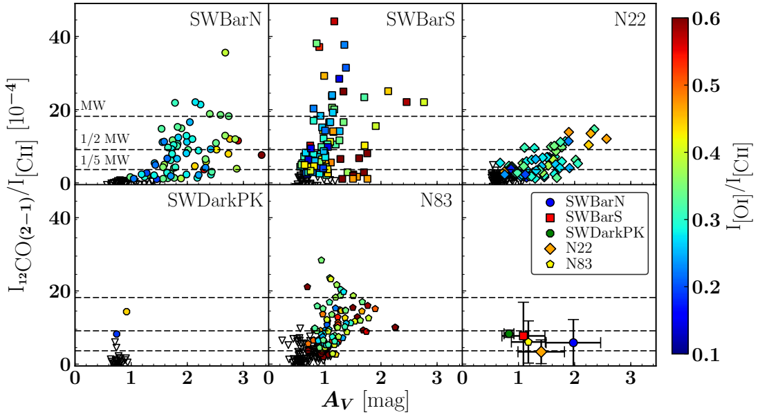
Figure 13. The ratio of the integrated intensity of ALMA ACA+TP ^{12}\text{CO} (2 – 1) to that of [C II] as a function of A_V for the HS 3 regions. The colored symbols show independent measurements detected at > 3\sigma in both ^{12}\text{CO} and [C II] the downward pointing triangles indicate upper limits (where I_{\text{CO}} < 3\sigma ). The over plotted dashed lines show scalings of the canonical [C II] to ^{12}\text{CO} (1 – 0) ratio translated to (2 – 1) assuming thermalized emission for the Milky Way of \sim 1/4400 (Stacey et al. 1991). The bottom left panel shows the mean ^{12}\text{CO} (2 – 1)/[C II] ratios for each region, which were calculated to include the upper limits (“left-censored” data) using the cenfit routine in the R package NADA (Lee 2017; Helsel 2005). We see a trend of ^{12}\text{CO} (2 – 1)/[C II] starting at values much lower than the Milky Way value at low A_V and increasing ^{12}\text{CO} (2 – 1)/[C II] towards higher A_V . The [O I]/[C II] ratios also show an increase towards higher A_V , which is consistent with increasing density producing more [O I] emission and/or less [C II].
