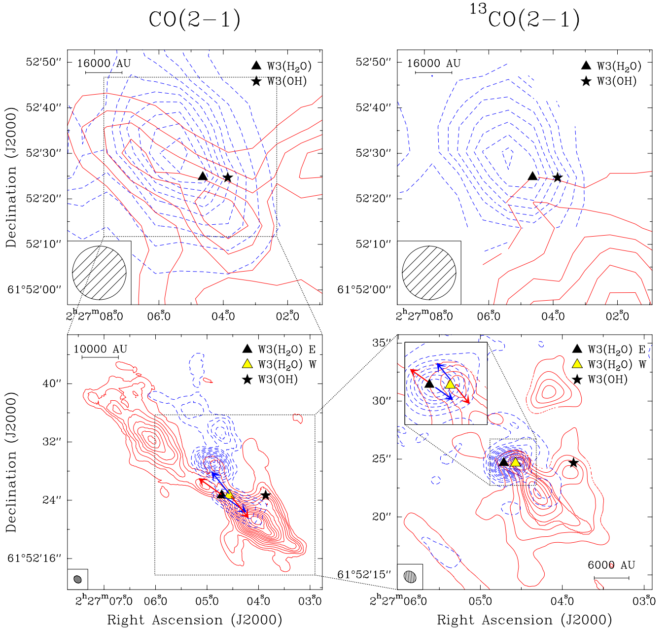
Fig. 6. Top left: Intensity map of CO (2–1) emission from IRAM 30-m integrated over the velocity range of -40 to -20 km s ^{-1} for the redshifted and -80 to -55 km s ^{-1} for the blueshifted gas. Contours start at 5\sigma and increase in steps of 5\sigma ( 1\sigma = 1.9 K km s ^{-1} ). Top right: Intensity map of ^{13}\text{CO} (2–1) emission from IRAM 30-m integrated over the velocity range of -40 to -20 km s ^{-1} for the redshifted and -80 to -55 km s ^{-1} for the blueshifted gas. Contours start at 3\sigma and increase in steps of 2\sigma ( 1\sigma = 0.42 K km s ^{-1} ). Bottom left: Intensity map of CO (2–1) emission obtained by Zapata et al. (2011) with the SMA integrated over the velocity range of -45 to -25 for the redshifted and -75 to -55 for the blueshifted gas. Contours start at 5\sigma and increase in steps of 5\sigma ( 1\sigma = 1.1 mJy beam ^{-1} km s ^{-1} ). The blue and red arrows highlight the positions and directions of the CO outflows emanating from each source. Bottom right: Intensity map of ^{13}\text{CO} (2–1) emission from IRAM 30-m merged with NOEMA observations integrated over the velocity range of -41 to -30 for the redshifted and -70 to -53 for the blueshifted gas. Contours start at 3\sigma and increase in steps of 3\sigma ( 1\sigma = 0.03 mJy beam ^{-1} km s ^{-1} for redshifted and 0.17 mJy beam ^{-1} km s ^{-1} for blueshifted sides). The zoom panel in the top left corner highlights the launching positions of each outflow, with the red and blue arrows showing the directions of the two bipolar outflows from Zapata et al. (2011). The rms noise used in drawing the contours of the integrated intensity maps have been determined by first creating the maps without any constraints on the minimum emission level (threshold of 0) and calculating the noise in an emission-free part of the resulting map.
