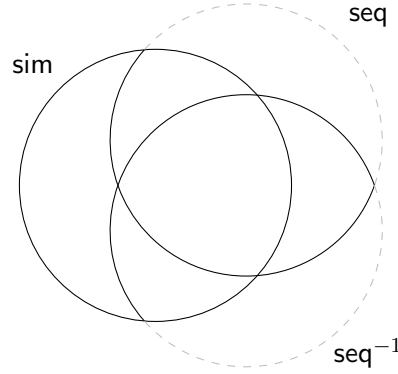
Figure 2: The relations defined by a step alphabet.
