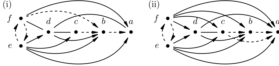
Figure 5: Dependence structure (i) sseq2or_{\theta_0}(u) and invariant structure (ii) or2ir(sseq2or_{\theta_0}(u)) of the step sequence u = (ef)dcba for the step alphabet \theta_0 from Figure 1. The relation \Rightarrow is depicted using solid (undirected) edges, \sqsubset by dashed arcs, and \prec = \Rightarrow \cap \sqsubset by solid arcs.
