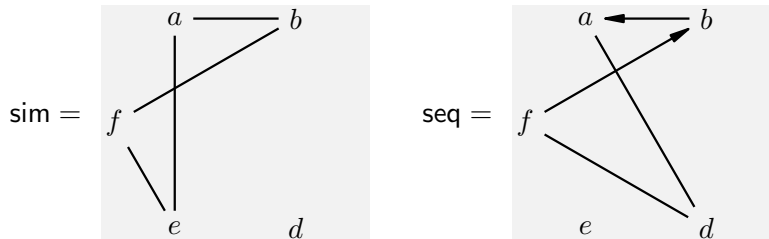
Figure 9: The step alphabet \theta_3 .
