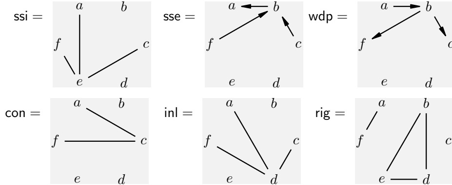
Figure 3: The partition of step alphabet \theta_0 .
