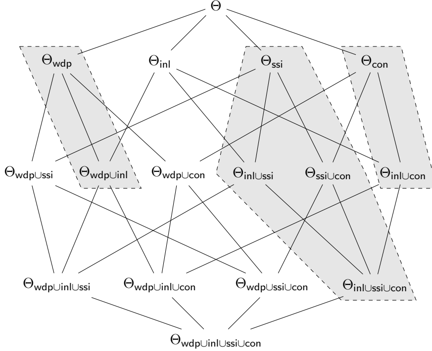
Figure 4: Hierarchy of the sixteen subclasses of step alphabets. When two classes are linked, the one higher up encompasses the lower one. The grey polygons show the three families of subclasses studied in Section 6.
