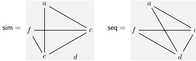
Figure 6: The step alphabet \theta_1 .
