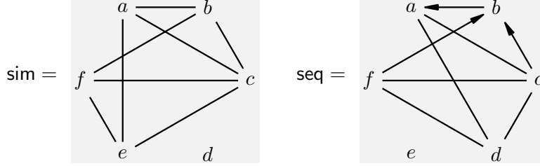
Figure 1: The step alphabet \theta_0 .
