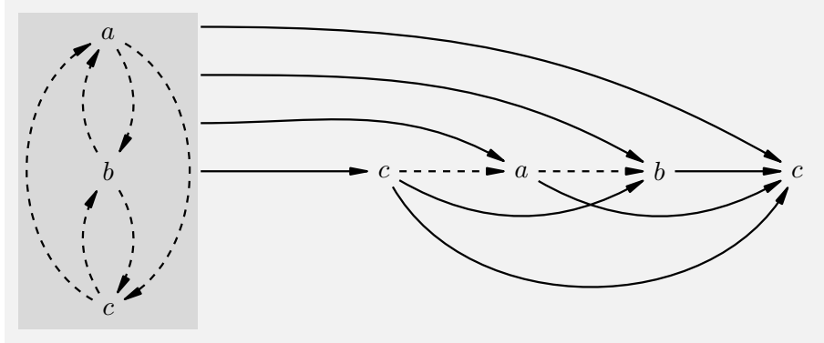
Figure 8: The invariant order structure ir of the step sequence (abc)cabc with the underlying occurrences ordered from left to right.
