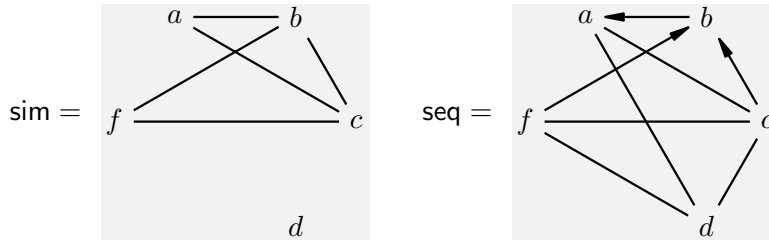
Figure 7: The step alphabet \theta_2 .
