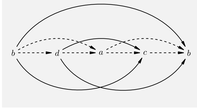
Figure 10: The invariant structure ir of bdacb with the underlying occurrences ordered from left to right.
