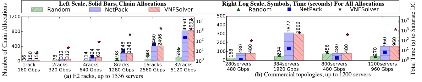
Figure 6: Runtime and total throughput achieved by RANDOM, NETPACK, and VNFSOLVER algorithms allocating 10-node VNF chain from Fig. 3e. Left. Allocating within DCs of the E2 [30] topology with increasing size (up to 1536 total servers). Right. Allocating the same chain in the commercial DCs of Section 5. Here, the largest DC has 1200 servers arranged in 60 racks. In both settings, NETPACK always achieves at least 96% of VNFSOLVER’s allocations, while completing in less than 2.5% of VNFSOLVER’s runtime.
