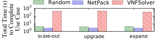
Figure 10: Use case completion time of scale-out , chain-upgrade , and expand on the commercial top. with 1200 servers. Operations are applied to an allocated abstract 4-node chain with 100 Gbps throughput.
