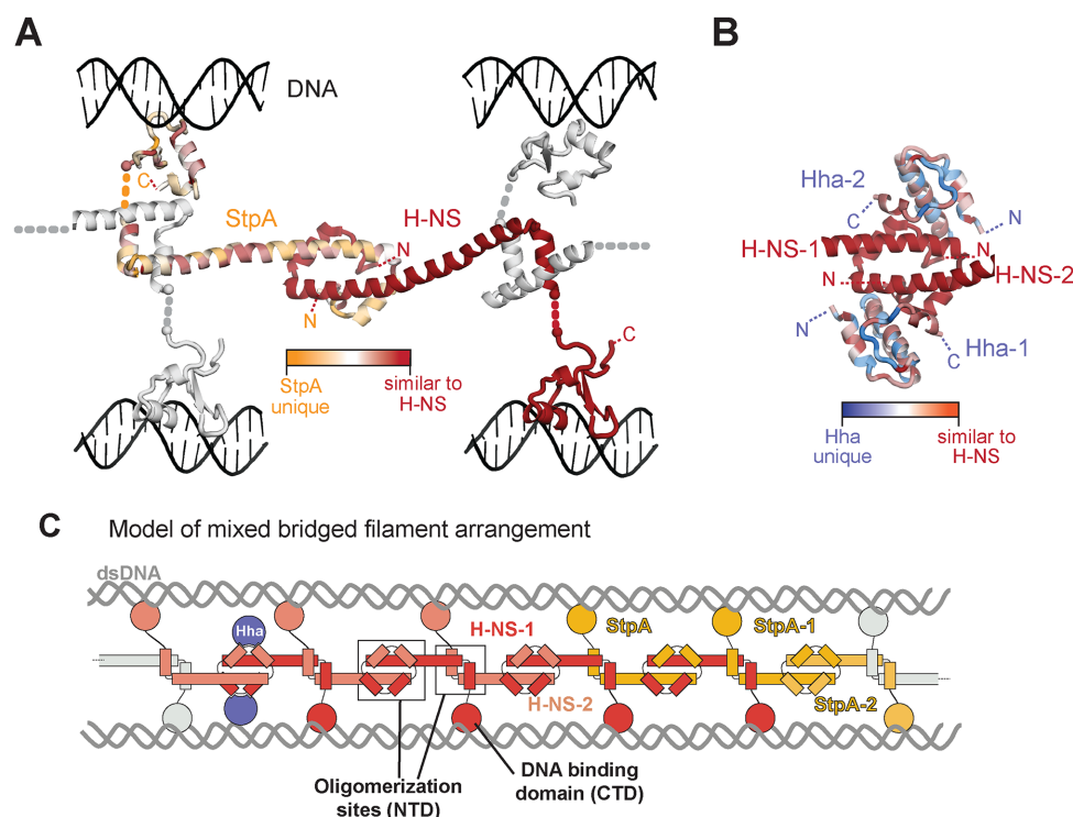
Figure 1. Structures and sequence similarities of H-NS, StpA and Hha. (A) StpA (orange/pink) modeled into the H-NS (red) head–head, tail–tail filament structure of the H-NS NTD (PDB ID: 3NR7; Ref. 57). Models of the StpA and H-NS CTDs interacting with DNA (DNA binding domain, DBD) are positioned to represent contacts in a bridged nucleoprotein filament based on an H-NS CTD structure (PDB ID: 1HNR; Ref. 99) and the H-NS paralog Ler CTD bound to DNA (PDB ID: 2LEV; Ref. 100). The StpA sequence conservation is shown as a color gradient of unique to StpA (orange) to similar to H-NS (red). StpA sequences from 26 species were aligned with H-NS to identify unique StpA residues and compared to H-NS to calculate sequence conservation (Supplementary Figure S1A and B). N and C indicate the N-terminus and C-terminus of proteins, respectively. (B) Hha sequence similarity compared to H-NS NTD is indicated by color gradient from red (similar to H-NS) to blue (unique to Hha) on both Hha monomers (Hha-1 and Hha-2) in the Hha:H-NS complex structure (PDB ID: 4ICG; Ref. 17). Although Hha is a member of the distinct YmoA protein family, it retains sequence similarity to H-NS. Hha sequences from 41 species were aligned with H-NS residues 1–83 to identify unique Hha residues (Supplementary Figure S1C). (C) Schematic adapted from Ref. (17) of the proposed arrangement of H-NS, StpA and Hha in a bridged nucleoprotein filament (H-NS, red and pink; StpA, yellow and pale yellow; Hha, blue; dsDNA, gray). The arrangement of H-NS, StpA and Hha in mixed nucleoprotein filaments is unknown.
