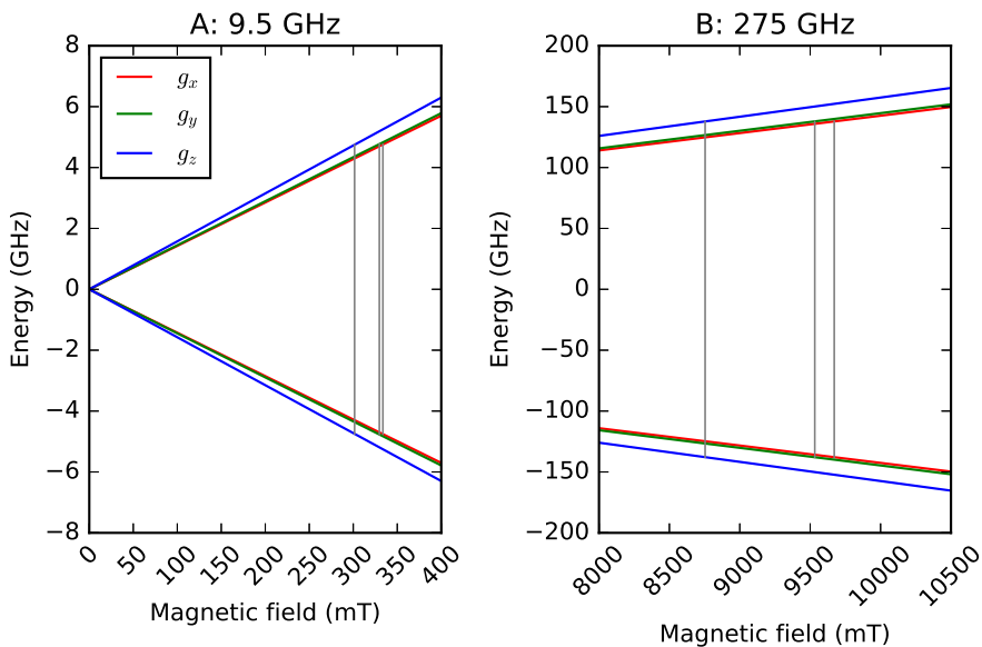
Figure 1.3: Simulated electron spin energy levels for an S = 1/2 system with anisotropic \mathbf{g} (whose x , y , and z components are represented in red, green, and blue, respectively), subjected to the Zeeman effect in the presence of an external magnetic field. (A) EPR transitions at the microwave frequency of 9.5 GHz (gray lines). (B) EPR transitions at the microwave frequency of 275 GHz (gray lines). The g -values g_x = 2.037 , g_y = 2.067 , and g_z = 2.25 are from [30]. Any other effect apart from the electron Zeeman is not included in the simulations, which are performed with EasySpin [31].
