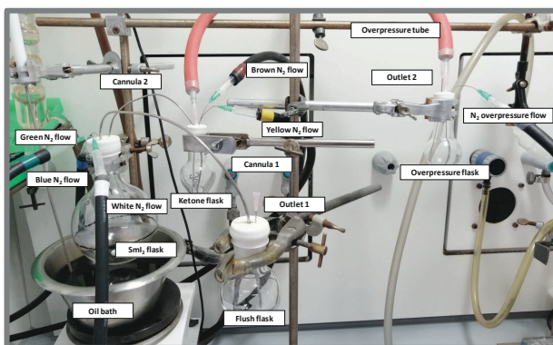
Figure S9. General setup of the SmI 2 -promoted C-C bond coupling.
