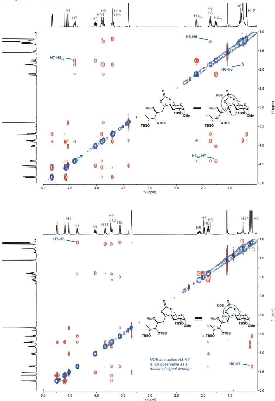
Figure S12. NOESY spectra of compound S29 and S30 . (A) The key NOE interactions for S29 can be found between \text{H3}_{\text{eq}} - \text{H7} and \text{H6} - \text{H8} . (B) The key NOE interaction for S30 can be found between \text{H6} - \text{H7} .
