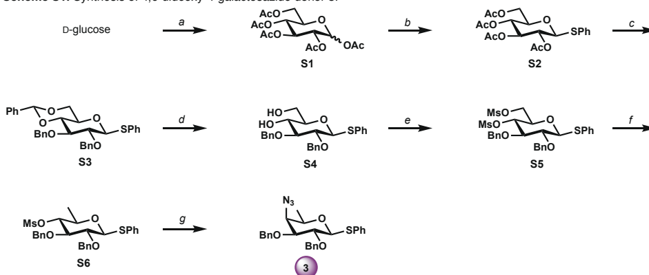
Scheme S1. Synthesis of 4,6-dideoxy-4-galactosazide donor 3.
