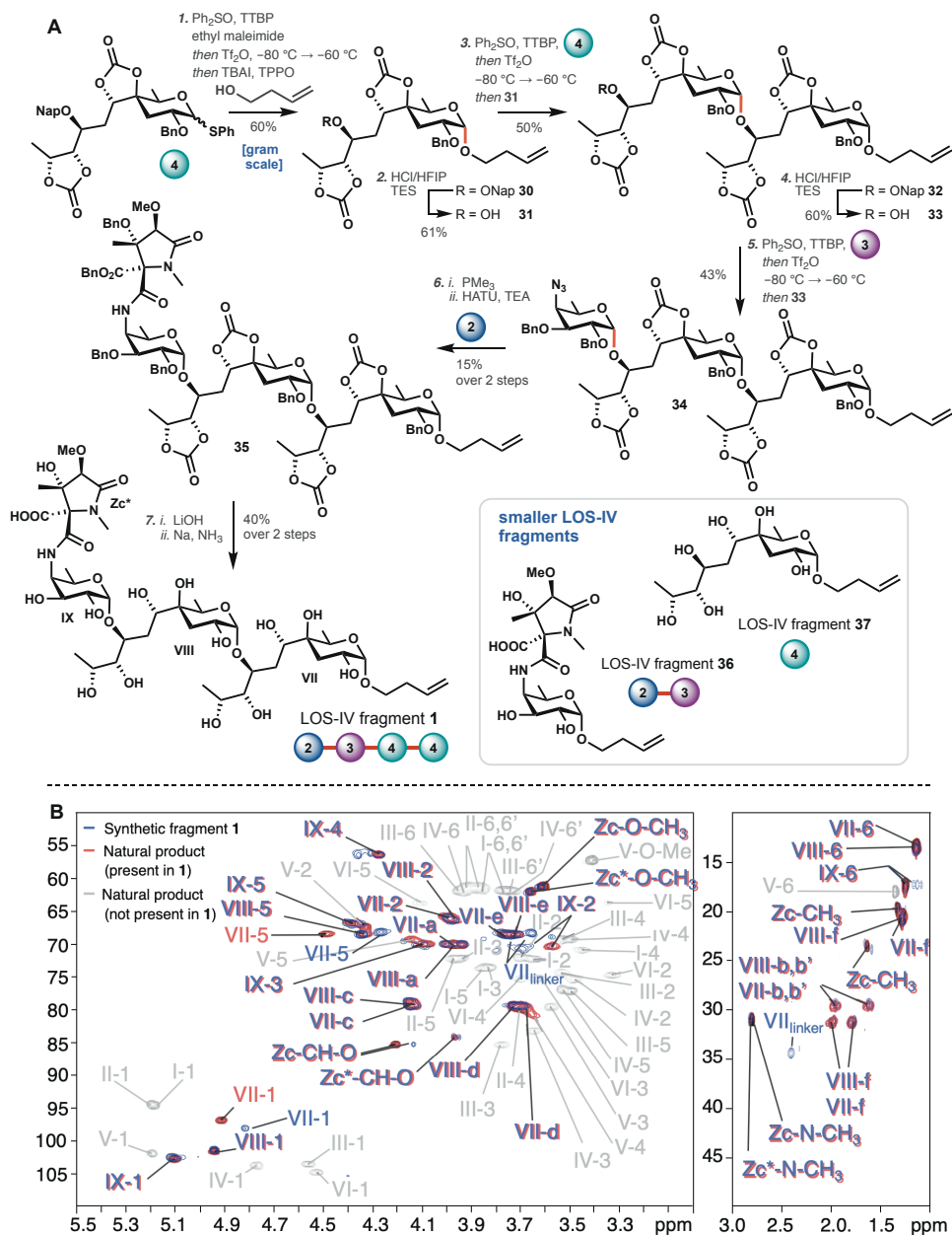
Figure 3. (A) Assembly of LOS-IV fragment 1. Reagents and conditions: (1) \text{Ph}_2\text{SO} , TTBP, N -ethyl maleimide, then \text{Ti}_2\text{O} , then TBAI, TPPO, then 3-buten-1-ol, -80^\circ\text{C} to 40^\circ\text{C} (60%); (2) HCl/HFIP, TES, DCM (61%); (3) \text{Ph}_2\text{SO} , TTBP, DCM, then \text{Ti}_2\text{O} , then 31, -80^\circ\text{C} to -60^\circ\text{C} (50%); (4) HCl/HFIP, TES, DCM (60%); (5) \text{Ph}_2\text{SO} , TTBP, DCM, then \text{Ti}_2\text{O} , then 33, -80^\circ\text{C} to -60^\circ\text{C} (43%); (6) i. trimethylphosphine, THF ii. 2, TEA, HATU, \text{CH}_3\text{CN} (15% over 2 steps); (7) i. LiOH, \text{H}_2\text{O} , THF ii. Na, \text{NH}_3 , t -BuOH, THF (40% over 2 steps); (B) ^1\text{H} - ^{13}\text{C} HSQC NMR overlay of the acidic OS-IV fraction isolated by Rombouts et al. (red = residues of the natural product present in the synthesized fragment 1, and grey = residues of the natural product absent in 1), and synthesized 1 (blue). I to IX correspond to the nine monosaccharides of the OS-IV. In the overlay most signals overlap. Only signals close to the linker on VII are slightly off, because this area is different from the natural compound, which is linked to a xylose.
