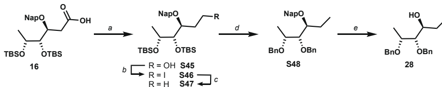
Scheme S7. Synthesis of compound 28.
