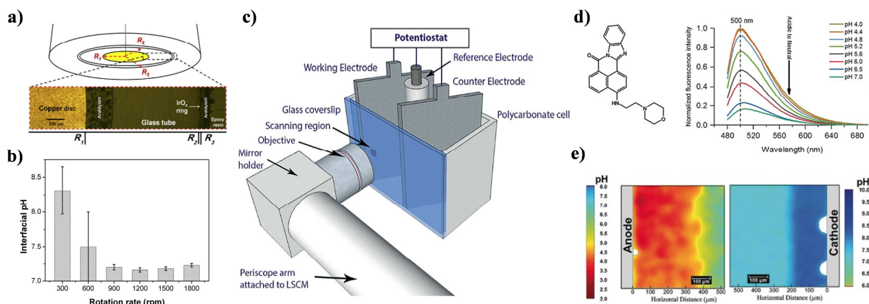
Figure 3. a) Schematic representation of an RRDE pH sensor and b) measurements performed with it during water reduction on copper at different rotation rates. Adapted with permission from [32]. Copyright (2015 Elsevier B.V. c) Schematic representation of a single compartment electrochemical cell coupled with a laser scanning confocal microscope, d) chemical structure of the LysoSensor Green DND-189 dye together with its normalized fluorescence response in phosphate buffer from pH 4 to 7, e) pH distribution at the anode and cathode during electrocoagulation, after a current density of 2 \text{ mA cm}^{-2} is applied for 60 s. Figures c, d and e are adapted from [46]. Copyright (2019) Wiley VCH Verlag GmbH & Co. KGaA.
