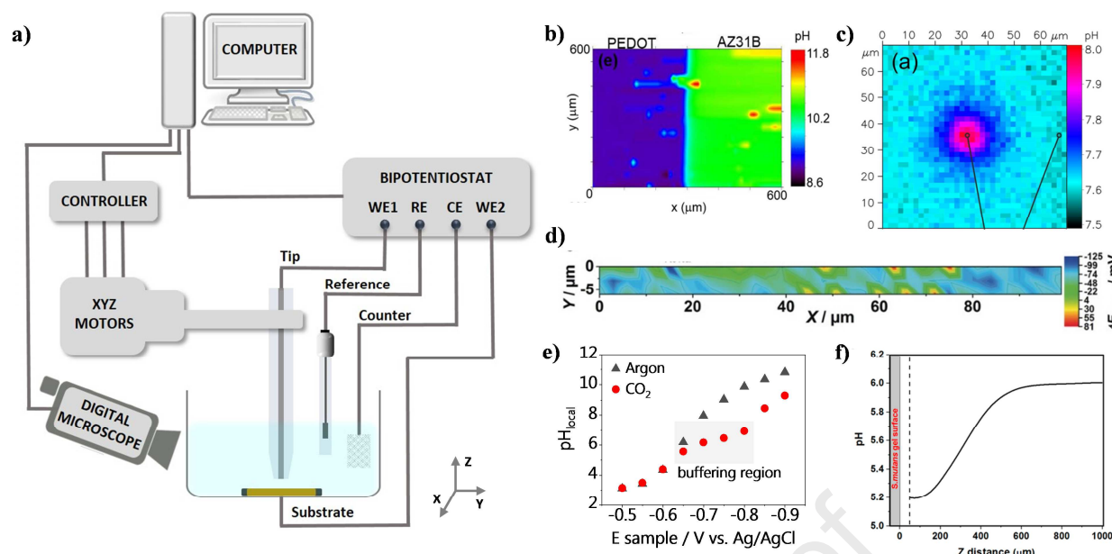
Figure 1. a) Schematic representation of a scanning probe setup, b) pH map of uncoated and PEDOT-coated AZ31B Mg alloy after 30 minutes in 0.01 M NaCl, measured with a Pt/IrOx microprobe operated in constant height potentiometric mode of SECM. Adapted from [8]. c) pH map during oxygen reduction on a 10 \mu\text{m} diameter Pt disc recorded with a voltammetric pH nanosensor made of a syringaldazine polymeric film. Adapted with permission from [15]. Copyright (2015) American Chemical Society. d) Image of the shifts in the reduction peak potential of a Pt nanoelectrode during oxygen reduction at a Ag-based gas diffusion electrode. Each grid point was measured at 1 \mu\text{m} tip-surface distance utilizing shear force constant distance mode SECM. Adapted with permission from [14]. Copyright (2018) Wiley- VCH Verlag GmbH & Co. KGaA. e) Buffering effect during \text{CO}_2 reduction measured with a voltammetric pH sensor based on a gold UME functionalized with a 4-NTP self-assembled monolayer. (M.C.O. Monteiro et al. unpublished). f) Z-directional pH profile recorded with a glass capillary filled with an ion-selective cocktail, from 50 \mu\text{m} above the S. mutans biofilm to 1000 \mu\text{m} in the bulk solution after addition of 30 mM sucrose in artificial saliva (pH 6.0). Adapted with permission from [23]. Copyright (2017) American Chemical Society.
