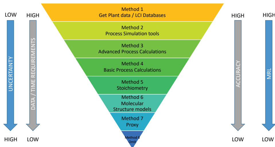
Figure 5.2: hierarchy of methods in LCI data generation adapted from Parvatker and Eckelman (2019).
