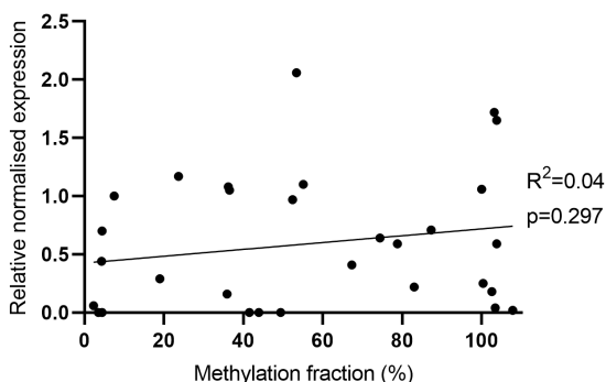
FIGURE 3. Correlation between methylation fraction (%) and TERT mRNA expression in total of 31 samples: fibroblasts (n=3), melanocytes (n=1), keratinocytes (n=2), cutaneous melanoma cell lines (n=19) and uveal melanoma cell lines (n=6). Linear regression and correlation analysis were performed to compare ( F_{(1,29)}=1.13 , r=0.19 , ns p=0.297 ).
