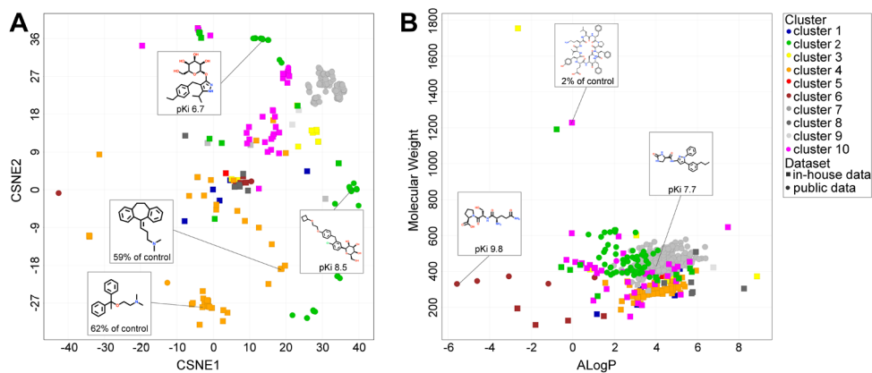
Figure 3.5. Clustering of hSGLT1 actives. Active hSGLT1 compounds in the training set clustered into ten chemical clusters (Tanimoto, FCFP6). Molecular structure and affinity (pKi for public data and % of (negative) control for in-house data) for representative cluster compounds are shown. In-house compounds with activity < 70% of (negative) control and public compounds with \text{pChEMBL} \geq 6.5 were used in clustering. A) t-SNE plot of the chemical clusters. B) the molecular weight and ALogP distribution of compounds in the chemical clusters.
