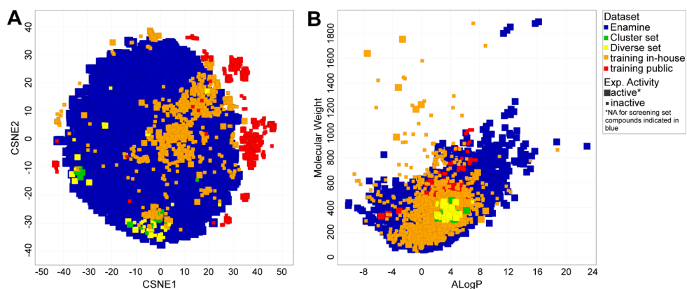
Figure 3.3. Chemical space of the selected compounds compared to the training and screening datasets. A) the Diverse set (yellow) and Cluster set (green) are displayed compared to the training (orange and red) and Enamine screening set (blue). The Enamine set is represented by a random selection of 20,000 out of the total of 1,815,674 compounds (~1%) in the screening set to limit t-SNE calculation time. B) the molecular weight and ALogP of the Diverse and Cluster set compared to the training and screening sets.
