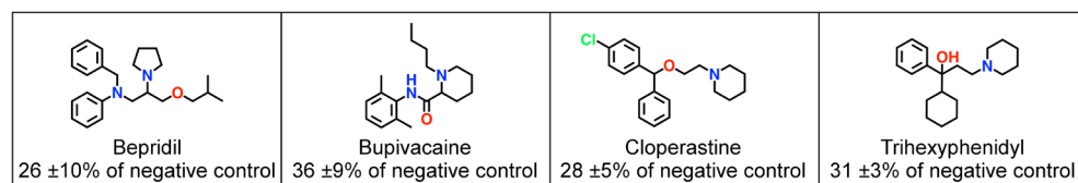
Figure 3.4. Reference hSGLT1 inhibitors for Cluster set and their inhibitory activity. Inhibitory activities (compared to negative control, where 100% is no inhibition) and chemical structures of four recently identified novel hSGLT1 inhibitors: bepridil, bupivacaine, cloperastine, and trihexyphenidyl.
