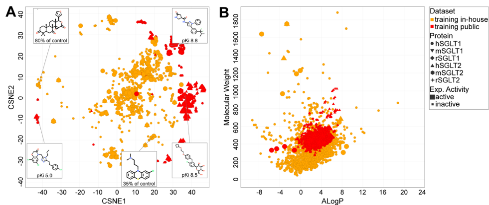
Figure 3.1. Chemical space of the public and in-house datasets. A) the t-SNE shows molecular structure and affinity ( pK_i for public data and % of (negative) control for in-house data) for representative hSGLT1 compounds. B) molecular weight and ALogP distribution of compounds in the training sets.
