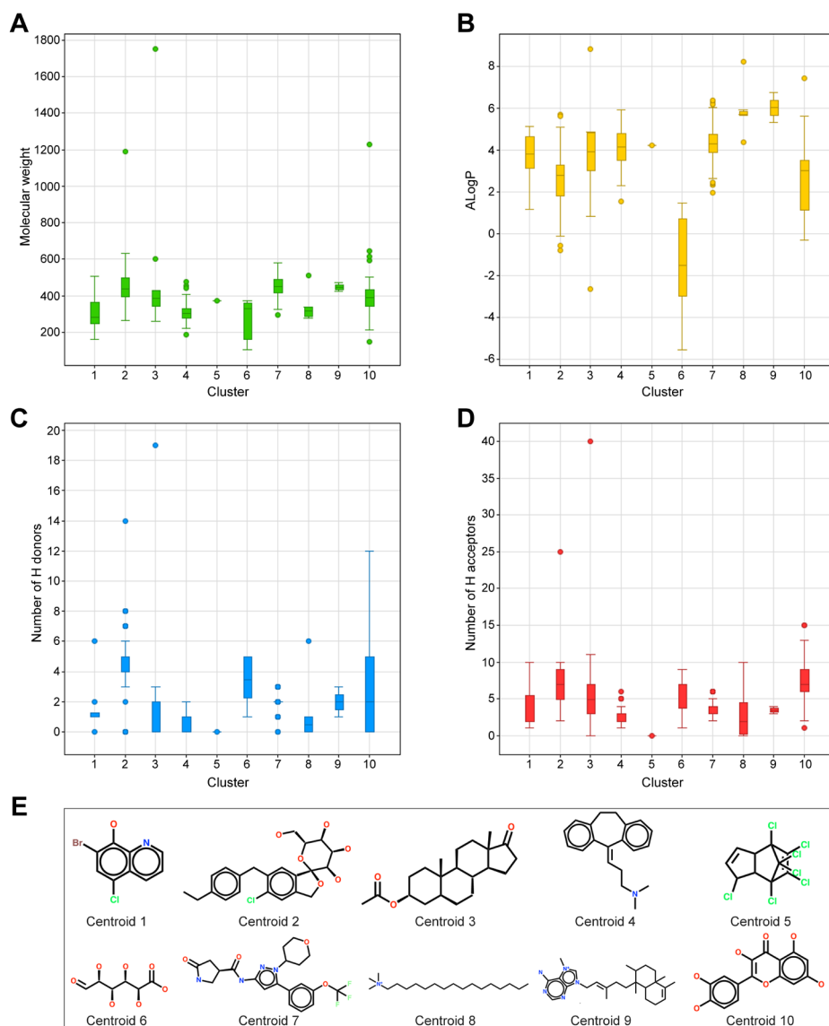
Figure 3.6. Cluster centers and distribution of physicochemical properties of hSGLT1 active compound clusters. Physicochemical properties of the ten clusters containing active hSGLT1 compounds. A) molecular weight. B) ALogP. C) number of hydrogen bond donors. D) number of hydrogen bond acceptors. E) molecular structures of the cluster centers.
