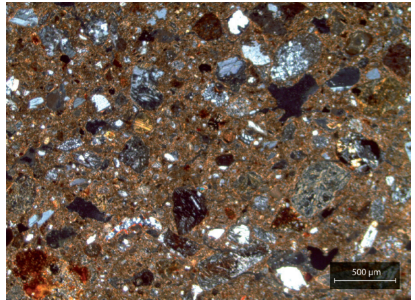
Figure 125: Example of a typical fabric for petrographic Group 7. Sample AB3.90 was photographed in XP (credit: Simone Casale).
