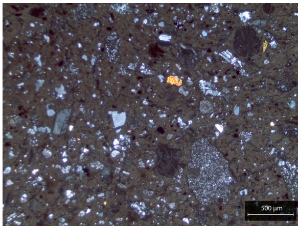
Figure 168: Example of a typical fabric for petrographic Group 5, featuring coarse inclusions with microphenocrysts of quartz, as well as single crystals of quartz, plagioclase, and amphibole. Sample OP1.85.S1 was photographed in XP (credit: Simone Casale).
