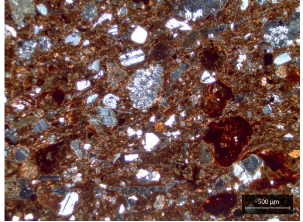
Figure 124: Example of a typical fabric for petrographic Group 6. Sample AB2.57.1 was photographed in XP (credit: Simone Casale).
