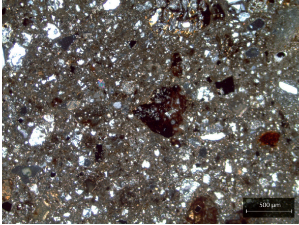
Figure 123: Example of a typical fabric for petrographic Group 5, a bimodal matrix featuring coarse intermediate extrusive volcanic rock inclusions with rare basalt in combination with smaller quartz and plagioclase feldspars. Sample AB2.35.S3 was photographed in XP (credit: Simone Casale).
