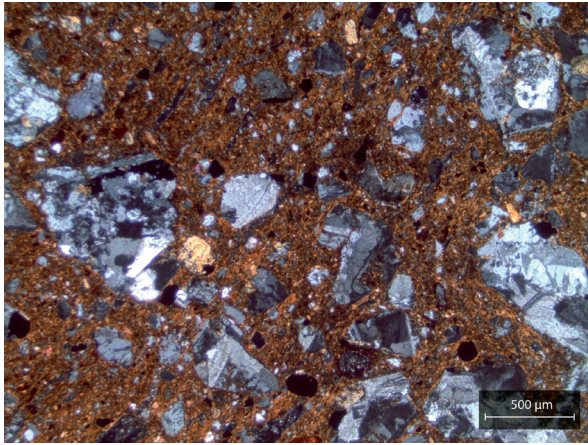
Figure 164: Example of a typical fabric for petrographic Group 1 featuring inclusions with large crystals connected to intrusive igneous rocks. Sample OP1.10.1 was photographed in XP (credit: Simone Casale).
