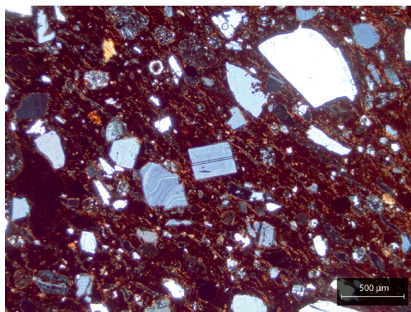
Figure 141: Example of a typical fabric for petrographic Group 1. Sample JOR2.S2(1) was photographed in XP (credit: Simone Casale).
