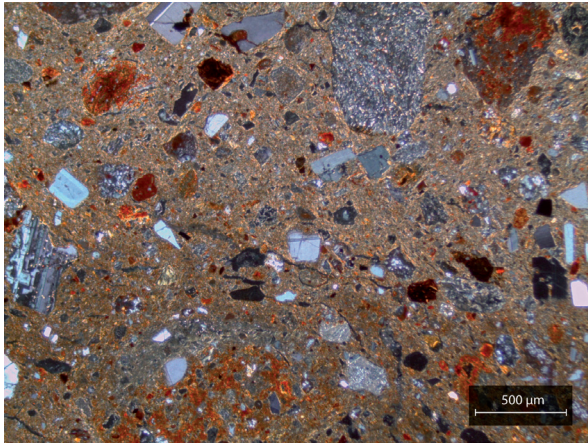
Figure 197: Sample RDO2.I2, featuring a matrix that was possibly sieved.
