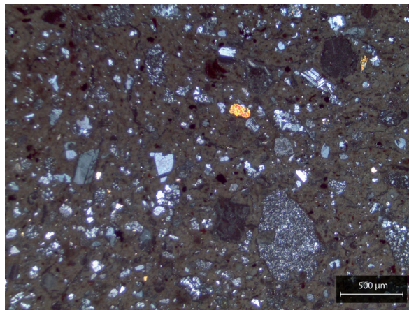
Figure 168: Example of a typical fabric for petrographic Group 5, featuring coarse inclusions with microphenocrysts of quartz, as well as single crystals of quartz, plagioclase, and amphibole. Sample OP1.85.S1 was photographed in XP (credit: Simone Casale).
