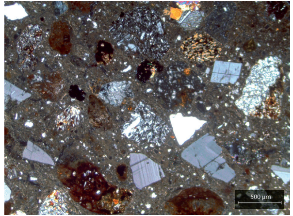
Figure 165: Example of a typical fabric for petrographic Group 2 featuring coarse volcanic rock inclusions, pyroxenes, plagioclase, and quartz. Sample OP1.139.2 was photographed in XP (credit: Simone Casale).
