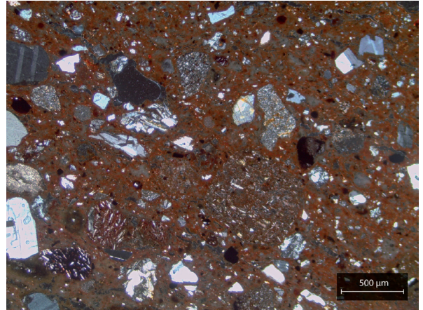
Figure 186: Example of a typical fabric for petrographic Group 2. Sample UBI3.W2 was photographed in XP (credit: Simone Casale).
