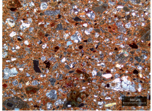
Figure 144: Example of a typical fabric for petrographic Group 3. Sample JOR2.RR4 was photographed in XP.
