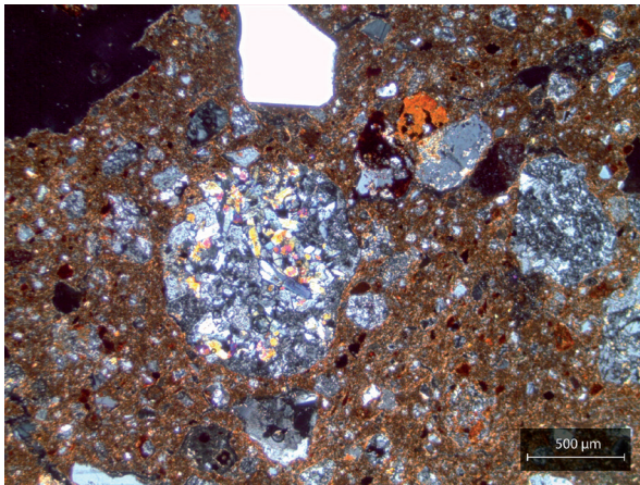
Figure 143: Example of a typical fabric for subgroup within petrographic Group 2 featuring volcanic and sedimentary rock inclusions. Sample JOR2.HH4 was photographed in XP (credit: Simone Casale).
