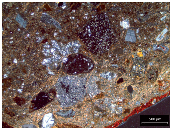
Figure 103: Example of petrographic Subgroup 1A, featuring coarse inclusions of granite, chert, and clay pellets. Sample AO1.6.5 was photographed in XP (credit: Simone Casale).
