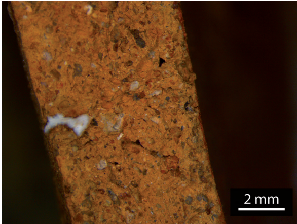
Figure 147: Example of oblique coil juncture visible on the cross-section (sample JOR2.59.1).
