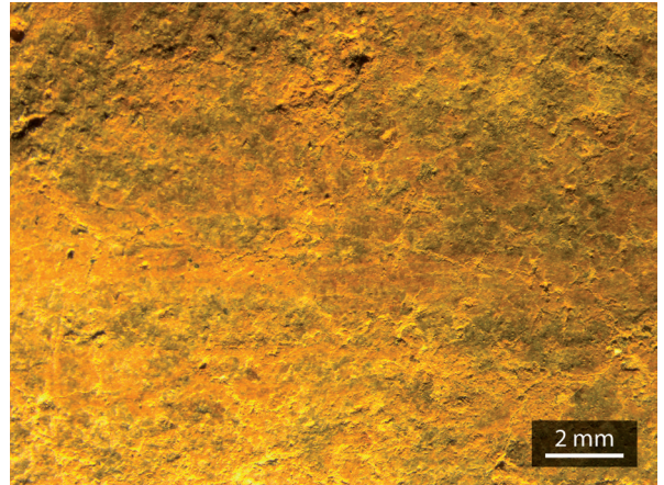
Figure 190: Sample UBI1CXIII5, featuring inserted grains, slip, and a burnished internal surface.
