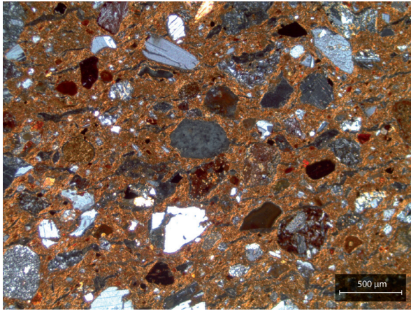
Figure 119: Example of a typical fabric for petrographic Group 1. Sample AB4.81b was photographed in XP (credit: Simone Casale).
