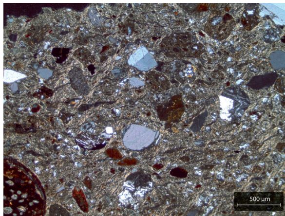
Figure 105: Example of petrographic Group 2, featuring andesite, sanidine, chert and clay pellets inclusions. Sample AO1.5.2 was photographed in XP (credit: Simone Casale).
