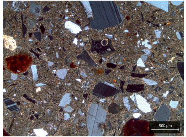
Figure 120: Example of a typical fabric for petrographic Group 2. Sample AB2.35.S2 was photographed in XP (credit: Simone Casale).
