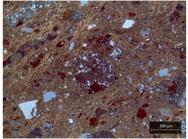
Figure 199: Example of a typical fabric for petrographic Group 2. Sample RDO1.E3 was photographed in XP (credit: Simone Casale).
