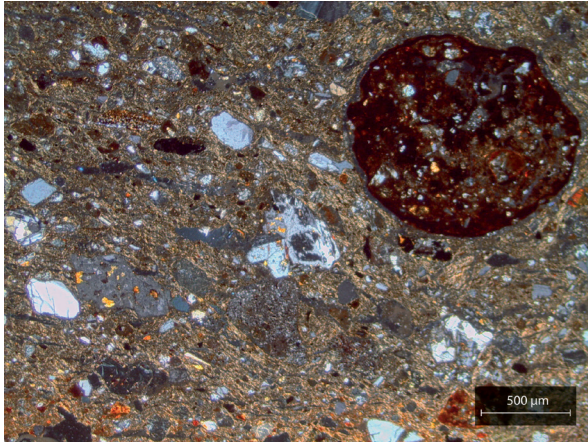
Figure 184: Example of a typical fabric for petrographic Group 3. Sample UBI1.H3 was photographed in XP (credit: Simone Casale).
