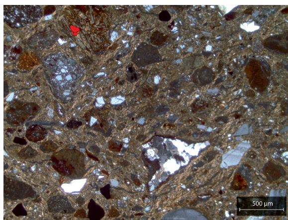
Figure 106: Subangular inclusions (i.e. granite) in petrographic Group 2. Sample AO1.6.1 was photographed in XP (credit: Simone Casale).
