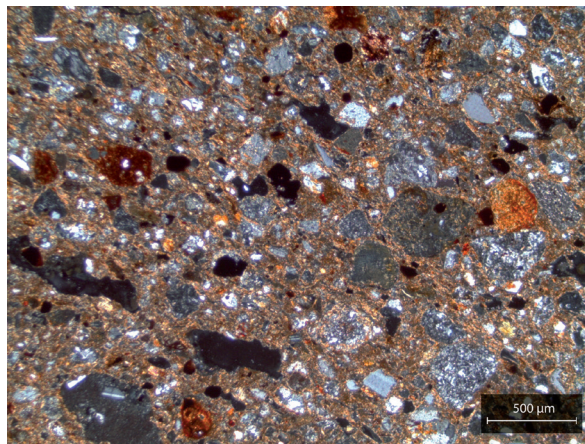
Figure 122: Example of a typical fabric for petrographic Group 4 featuring rock fragments, voids, clay pellets, quartz, plagioclase, and iron-rich inclusions. Sample AB2.57.3 was photographed in XP (credit: Simone Casale).
