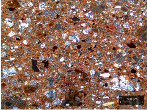
Figure 142: Example of a typical fabric for petrographic Group 2. Sample JOR2.FF4(2) was photographed in XP.
