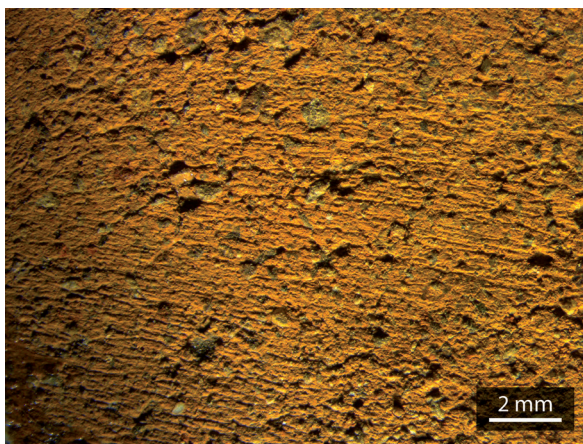
Figure 127: Wet clay traces (prominent grains combined with threaded striations), internal surface of sample AB2.35.S3.
