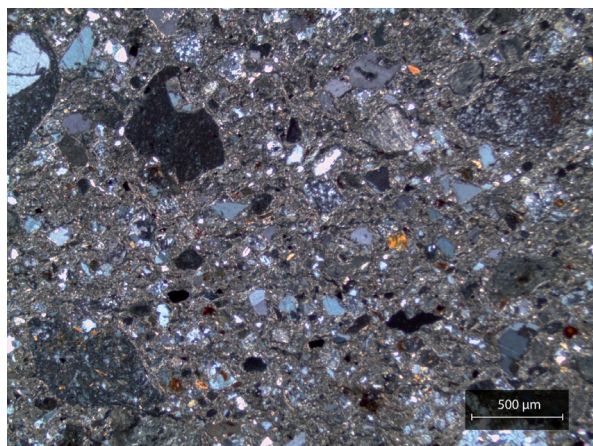
Figure 200: Example of a typical fabric for petrographic Group 3. Sample RDO1.E1 was photographed in XP.
