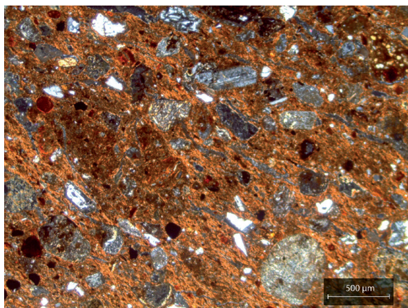
Figure 102: Example of a typical fabric for petrographic Group 1. Sample AO1.5.12 was photographed in XP (credit: Simone Casale).
