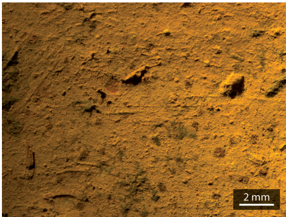
Figure 189: Sample UBI1B.9, featuring prominent grains covered by coating.
