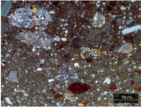
Figure 107: Petrographic Group 3 featuring granite, clay pellets, chert, and quartz inclusions. Sample AO1.6.4 was photographed in XP (credit: Simone Casale).
