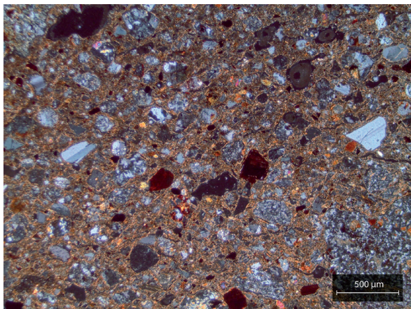
Figure 167: Example of a typical fabric for petrographic Group 4. Sample OP1.169.1 was photographed in XP (credit: Simone Casale).
