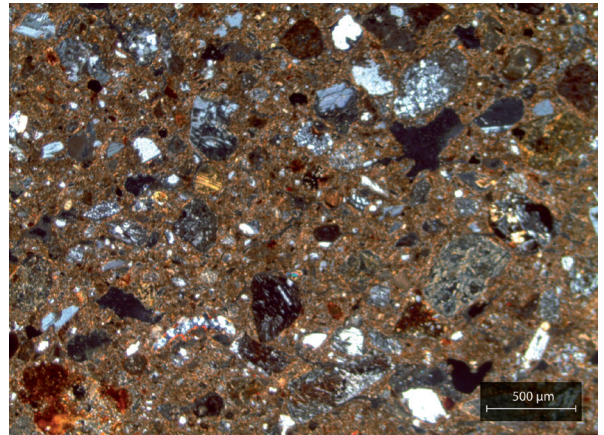
Figure 125: Example of a typical fabric for petrographic Group 7. Sample AB3.90 was photographed in XP (credit: Simone Casale).
