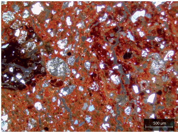
Figure 198: Example of a typical fabric for petrographic Group 1. Sample RDO1.X4 was photographed in XP (credit: Simone Casale).
