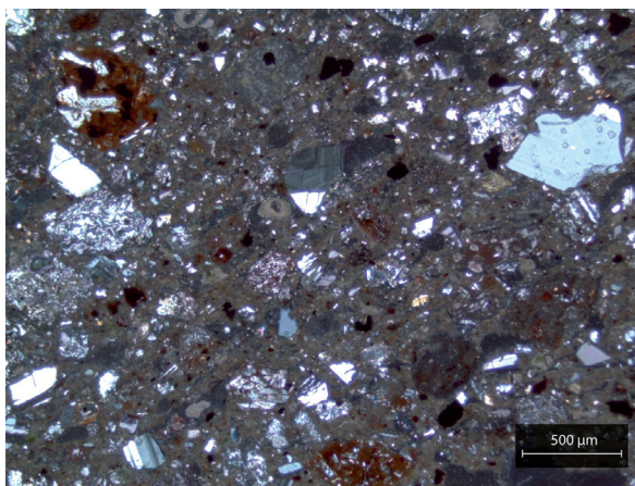
Figure 213: Example of a typical fabric for petrographic subgroup Group 1, featuring quartz and feldspar tempering. Sample LA1.B4 was photographed in XP.
