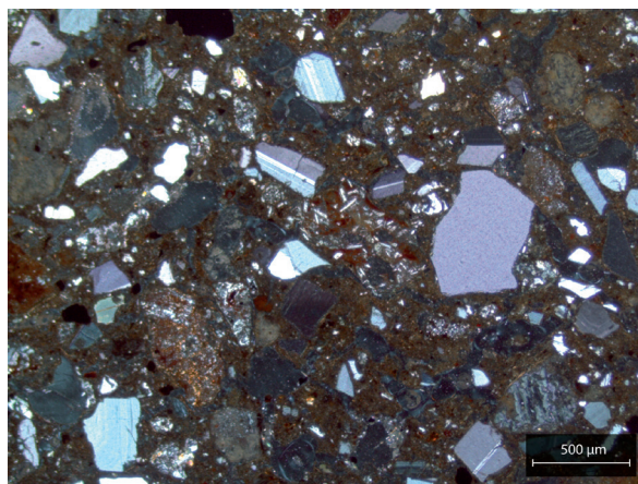
Figure 182: Example of a typical fabric for petrographic Group 1. Sample UBI1.B4.3 was photographed in XP (credit: Simone Casale).
