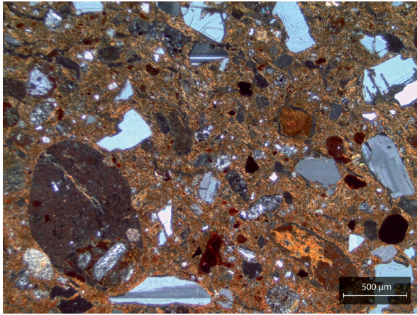
Figure 183: Example of a typical fabric for petrographic Group 4. Sample UBI1.BB1 was photographed in XP (credit: Simone Casale).
