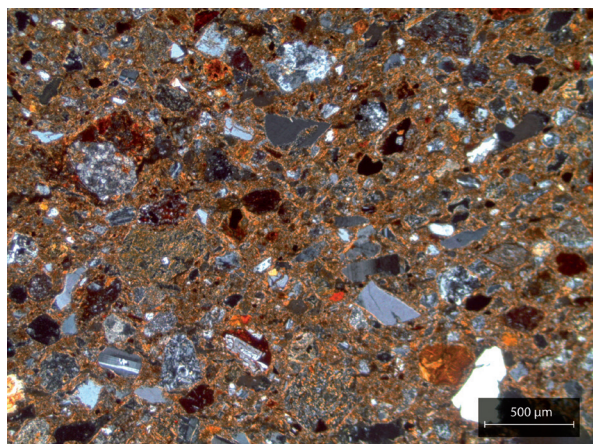
Figure 224: Thin section of a modern griddle, produced by the Güegüestepe community of potters. Sample was photographed in XP (credit: Simone Casale).
