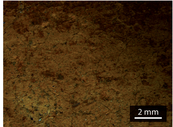
Figure 204: Sample RDO1.E1, featuring inserted grains and compact microtopography, characteristic of leather hard clay smoothing.
