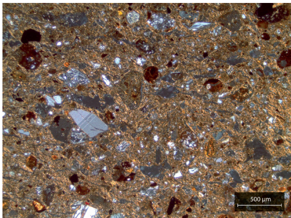
Figure 104: Example of petrographic Subgroup 1B. Sample AO1.5.3 was photographed in XP (credit: Simone Casale).
