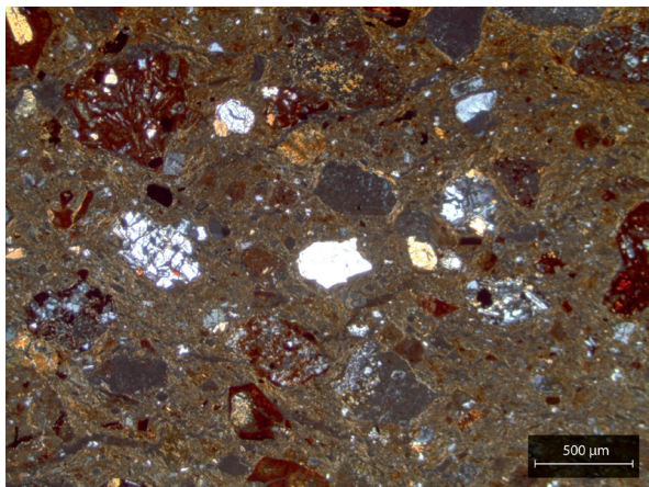
Figure 121: Example of a typical fabric for petrographic Group 3. Sample AB5.173 was photographed in XP (credit: Simone Casale).
