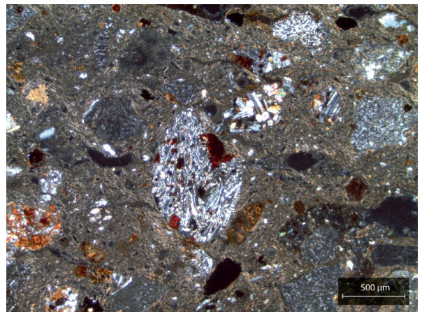
Figure 166: Example of a typical fabric for petrographic Group 3 featuring basalt inclusions with magnetite and titanate, as well as yellow pale olivine. Sample OP1.159 was photographed in XP (credit: Simone Casale).
