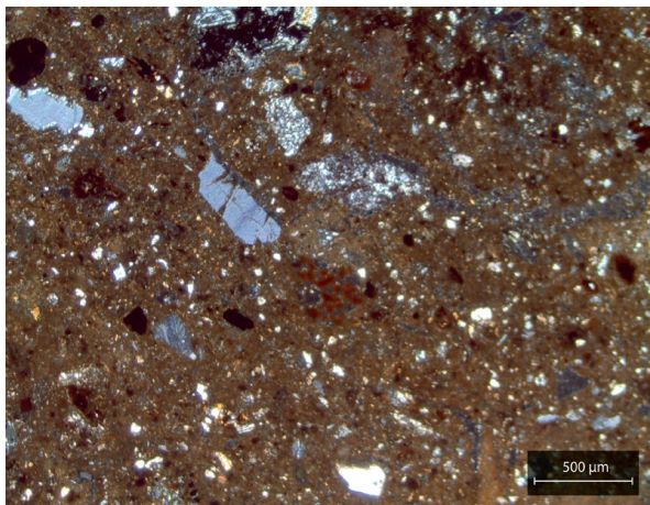
Figure 187: Example of a typical fabric for petrographic Group 6. Sample UBI1.FF1 was photographed in XP (credit: Simone Casale).
