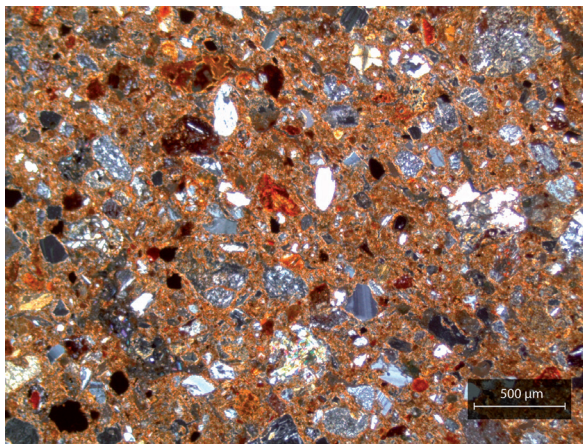
Figure 212: Example of a typical fabric for petrographic Group 1. Sample LA1.A4(8) was photographed in XP.
