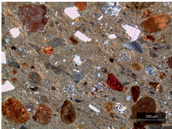
Figure 145: Example of a typical fabric for subgroup within petrographic Group 3. Sample JOR2.E1 was photographed in XP.
