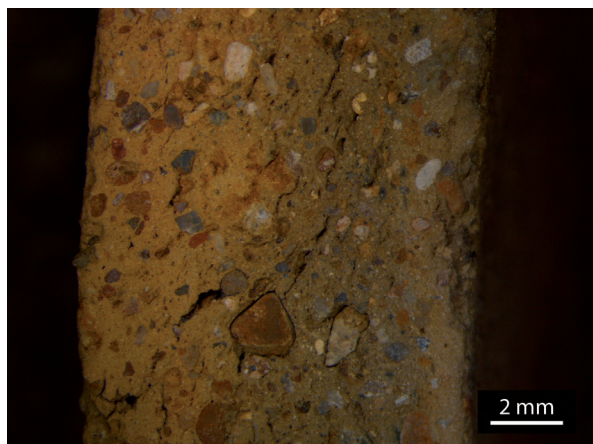
Figure 126: Cross-section from the ceramic assemblage EAB2 featuring coils.
