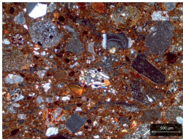
Figure 169: Example of a typical fabric for petrographic Group 6, featuring an alkali-based olivine-rich basalt inclusion, together with volcanic inclusions with microphenocrysts of feldspars. Sample OP1.169.2 was photographed in XP (credit: Simone Casale).
