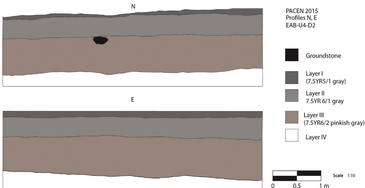
Figure 37: Drawing of Aguas Buenas excavation unit 4 (EAB4) northern and eastern profiles.
