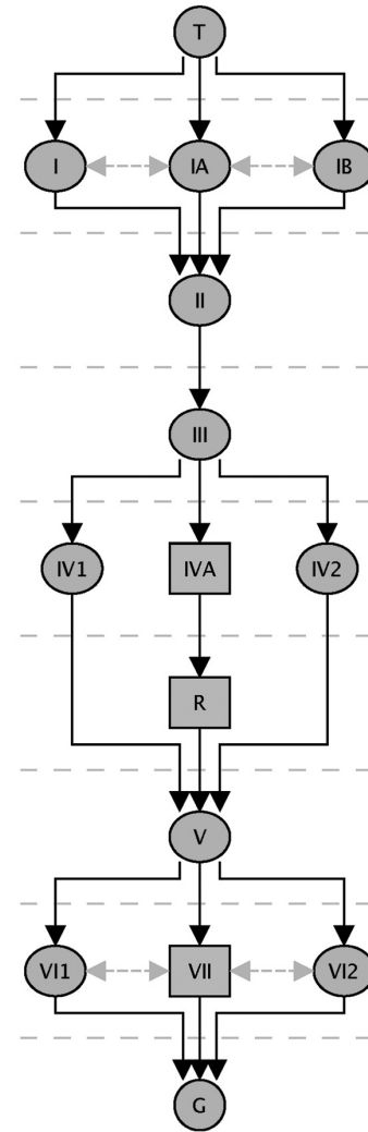
Figure 74: Harris matrix model for Josefa Ocón Robleto excavation unit 2 (EJOR2).
