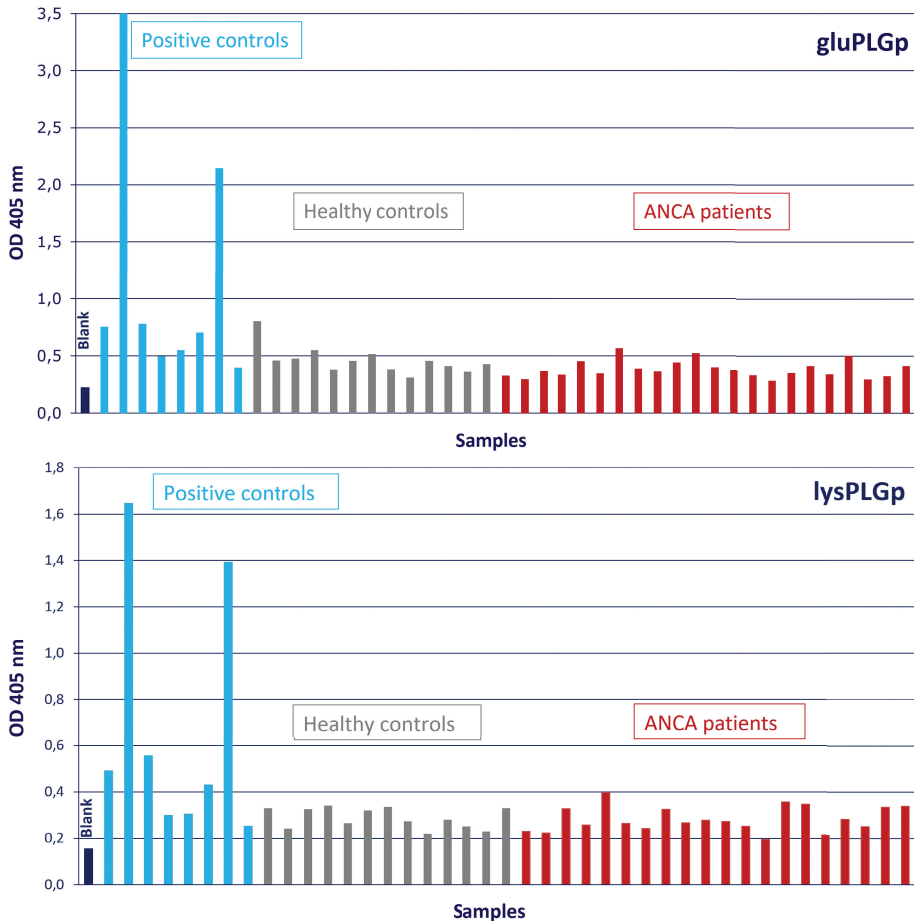
Figure 2 | Spectrophotometrical results.
