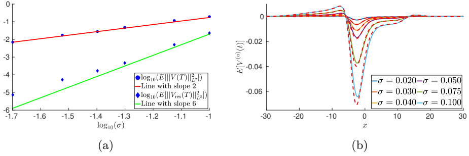
Figure 4.14: Panel (a) is computed from Figure 4.12 by evaluating the expectations at the last time step T = 1000 and plotting them as function of \sigma . We observe that E[||V(T)||^2_{L^2(\mathbb{R}, \mathbb{R}^2)}] scales as \mathcal{O}(\sigma^2) as predicted and E[||V_{\text{res}}(T)||^2_{L^2(\mathbb{R}, \mathbb{R}^2)}] scales significantly faster then \mathcal{O}(\sigma^4) , but not as the predicted \mathcal{O}(\sigma^6) . Panel (b) is computed from Figure 4.13, by evaluating E[V^{(u)}(50)] . The dashed lines correspond to the second order predictions \sigma^2 E[V_0^{(u,2)}(50)] .
