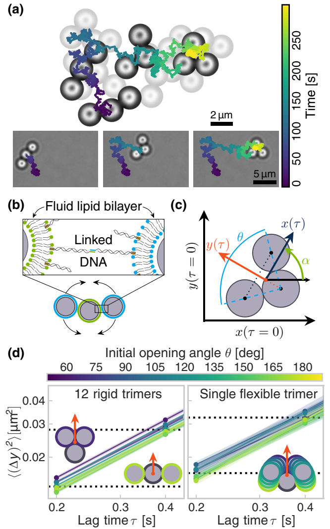
FIG. 1. Diffusion of flexible trimers. (a) Overlay of bright-field microscopy images of a flexible trimer with the position of its center of mass as function of time. (b) Schematic (not to scale) of flexible trimers that are self-assembled from colloidal supported lipid bilayers. We inserted DNA linkers into the fluid lipid bilayer surrounding the particle, resulting in bonded particles that can rearrange with respect to each other. (c) Illustration of the body-centered coordinate system. (d) The mean squared displacement of rigid and flexible trimers. The translational mean-squared displacement of flexible trimers in the y -direction is angle dependent for short lag times, at longer lag times this angle dependence is no longer present due to rotational and conformational relaxation, which happens on a shorter timescale than for rigid trimers (raw data, not scaled with friction coefficients).
