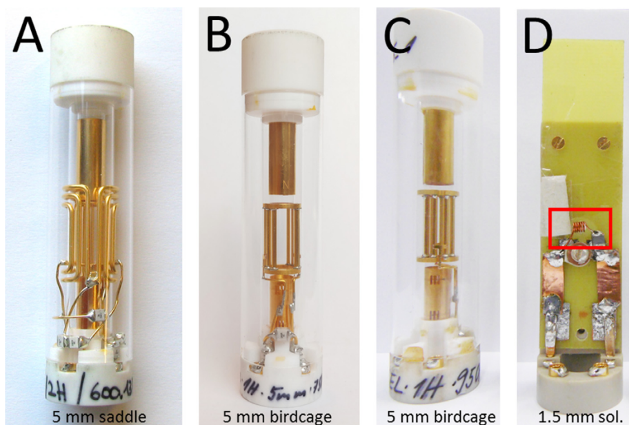
Fig. 1. The exchangeable coil inserts of the different spectrometers are shown. A.) On the 14.1 T spectrometer, a 5 mm 1\text{H}/^2\text{H} dual insert was used with the inner coil being the ^1\text{H} - saddle coil. B.) The 17.6 T spectrometer was equipped with a 5 mm birdcage coil and C.) for the 22.3 T spectrometer a 5 mm birdcage and D.) a home-built 1.5 mm solenoid coil (red highlight) was used.
