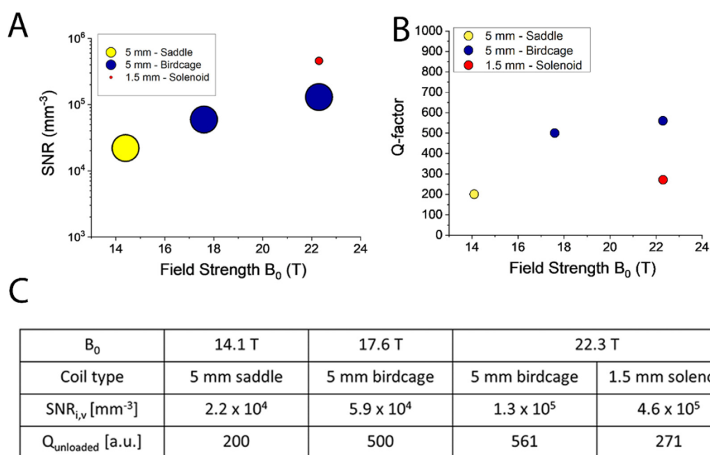
Fig. 2. A) Signal-to-Noise Ratio for different coils at 14.1 T, 17.6 T and 22.3 T shows an \text{SNR}_{i,v} increase for the 5 mm volume coils with an increase of B_0 field and an \text{SNR}_{i,v} increase for the 1.5 mm solenoid compared to the 5 mm birdcage (@ 22.3 T). B) The Q-factor of all available coils of the different spectrometers were determined. C) All numerical quantities as depicted in A and B are listed.
