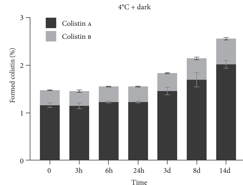
FIGURE 2 Time course of ratio colistin A to colistin B in elastomeric infusion pumps containing colistin methanesulphonate in 100 ml 0.9% saline when stored under different conditions.
