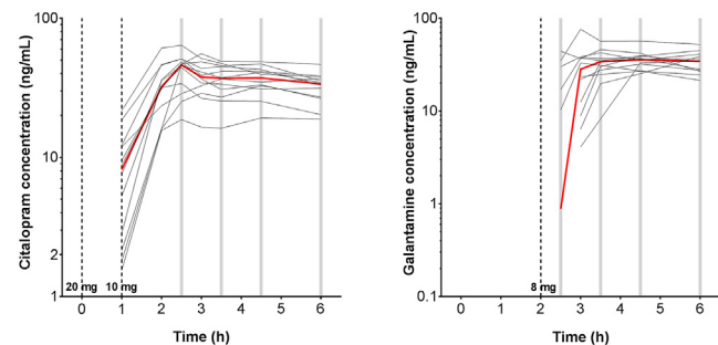
Fig. 2. Pharmacokinetic profiles. Median (red line) and individual (black lines) PK profiles for citalopram (left) and galantamine (right) concentrations in AD patients (a) and controls (b). Vertical bars illustrate the timing of RS-fMRI acquisition post drug administration. Observations below limit of quantification were dismissed.
