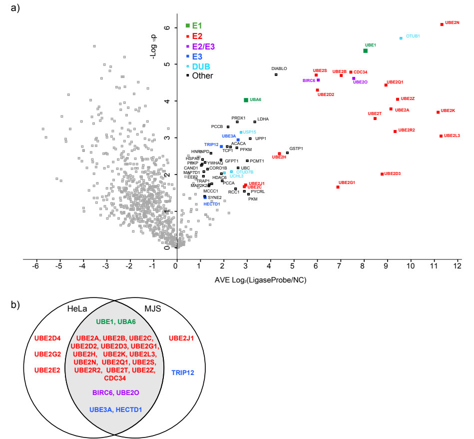
Supplementary Figure 16. Proteome-wide activity profiling of the Ub conjugation machinery in MeJJuSo cells. a) Volcano plot of pairwise comparison of proteins bound to the Biotin-UbDha probe relative to the apyrase-treated negative control (negative log 10 p-value, y-axis) as a function of average log 2 fold enrichment (x-axis). Colored dots represent confidently identified Ubiquitin machinery components as follows: E1 (green), E2 (red), HECT E3 (blue), hybrid E2/E3 (purple) and DUBs (light blue), with an average log 2 ratio greater than 1 and with p < 0.05 . Hits unrelated to the Ub cycle are marked in black, and proteins falling below the threshold are shown in gray. b) Venn diagram of shared Ub-conjugation enzymes recovered from HeLa and MeJJuSo cells.
