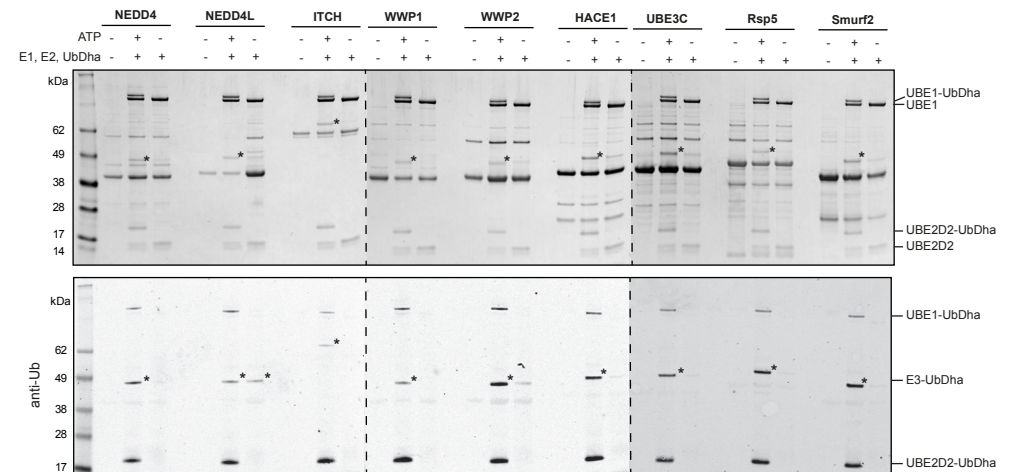
Supplementary Figure 7. UbDha shows reactivity towards E3 HECT enzymes under ATP dependent conditions. The asterisks indicate the E3-UbDha thioether-linked adduct. Visualized by silver staining (upper panel) and western blot against Ub (lower panel).
