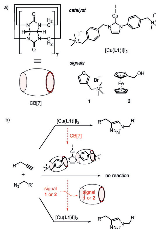
Figure 1. a) Structure of cucurbit[7]uril (CB[7]) and molecular structure of the Cu I –NHC catalyst [\text{Cu}(\text{L1})]\text{I}_2 and signal molecules 1 and 2. b) When [\text{Cu}(\text{L1})]\text{I}_2 is encapsulated by CB[7], catalytic activity in the CuAAC is “switched off”. After the addition of the signal molecule 1 or 2, [\text{Cu}(\text{L1})]\text{I}_2 is released, which “switches on” the catalytic activity.
