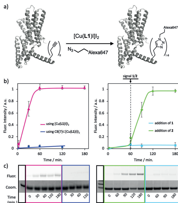
Figure 3. a) [Cu(L1)]I 2 -catalyzed fluorescence labeling of alkyne-handle-modified vinculin protein with azide-Alexa 647. The recombinant vinculin protein has eight alkyne groups at various positions in its structure. b) Left: Relative conversion of fluorescence labeling over time. Uninhibited fluorescence labeling reached its maximum value after approximately 60 min (magenta), whereas no significant conversion was observed for CB[7]-inhibited fluorescence labeling over the course of 120 min (blue). Right: Activation of fluorescence labeling using signal molecules. No catalyst activation was observed when signal molecule 1 was added after 60 min (dashed line) to a sample with the CB[7]-inhibited catalyst (cyan). In a similarly inhibited sample, the addition of signal molecule 2 after 60 min led to immediate fluorescence labeling (green). Lines have been drawn to guide the eye. c) Scans of gels stained with Coomassie (Coom.) and analyzed for fluorescence intensity (Fluor.) over time (min). Coomassie bands shown in the black frames indicate the 40 kDa protein marker (recombinant vinculin MW is 35.6 kDa (453–724 amino acid sequence of wild-type vinculin)).
